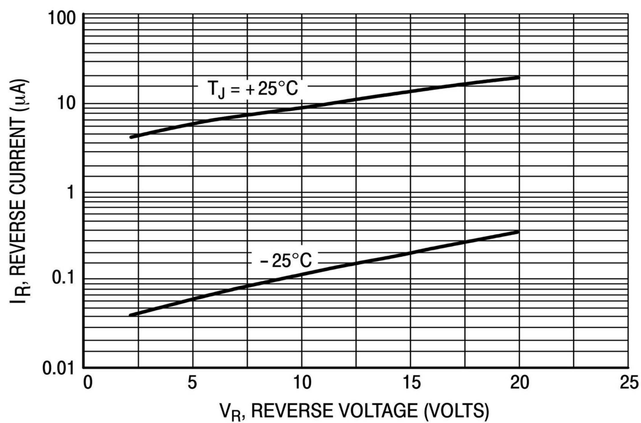
Figure 4. Typical Reverse Current
