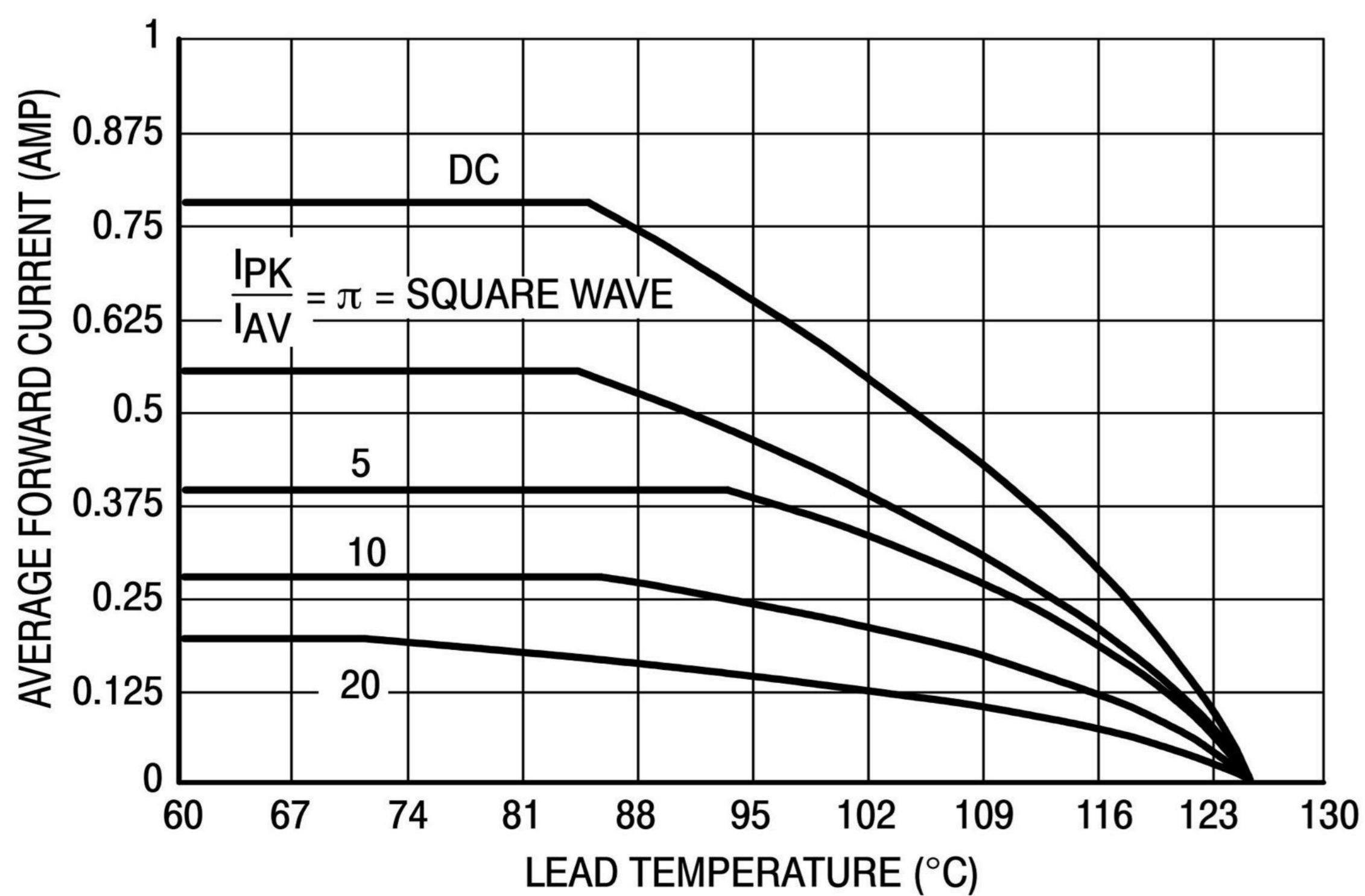
Figure 5. Current Derating (Lead)
