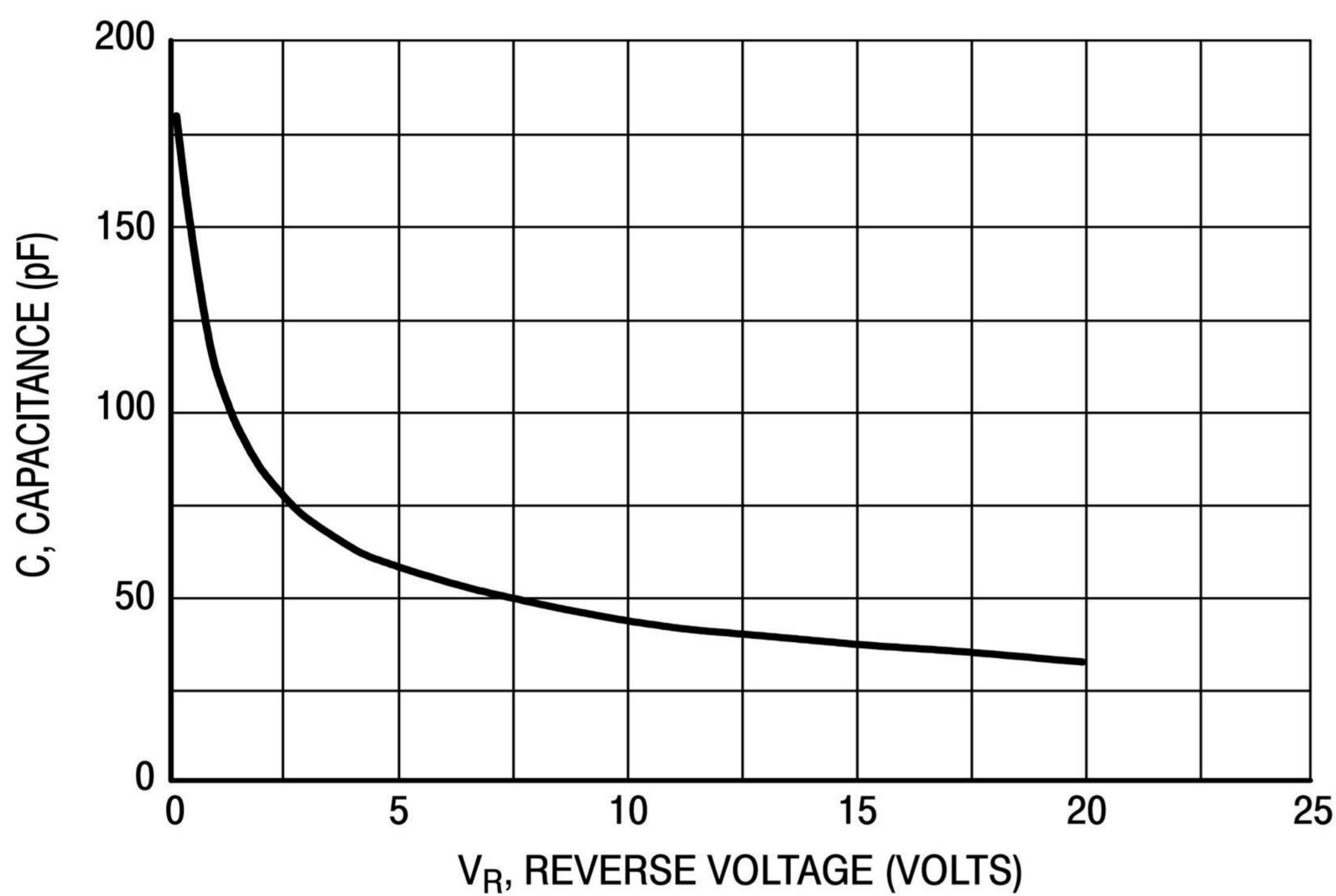
Figure 3. Typical Capacitance
