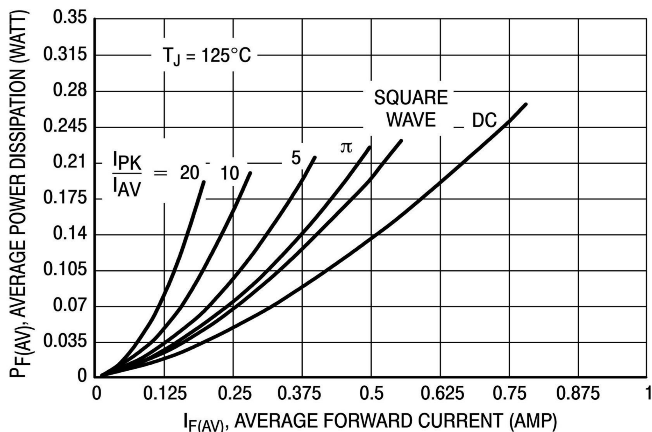
Figure 6. Power Dissipation
