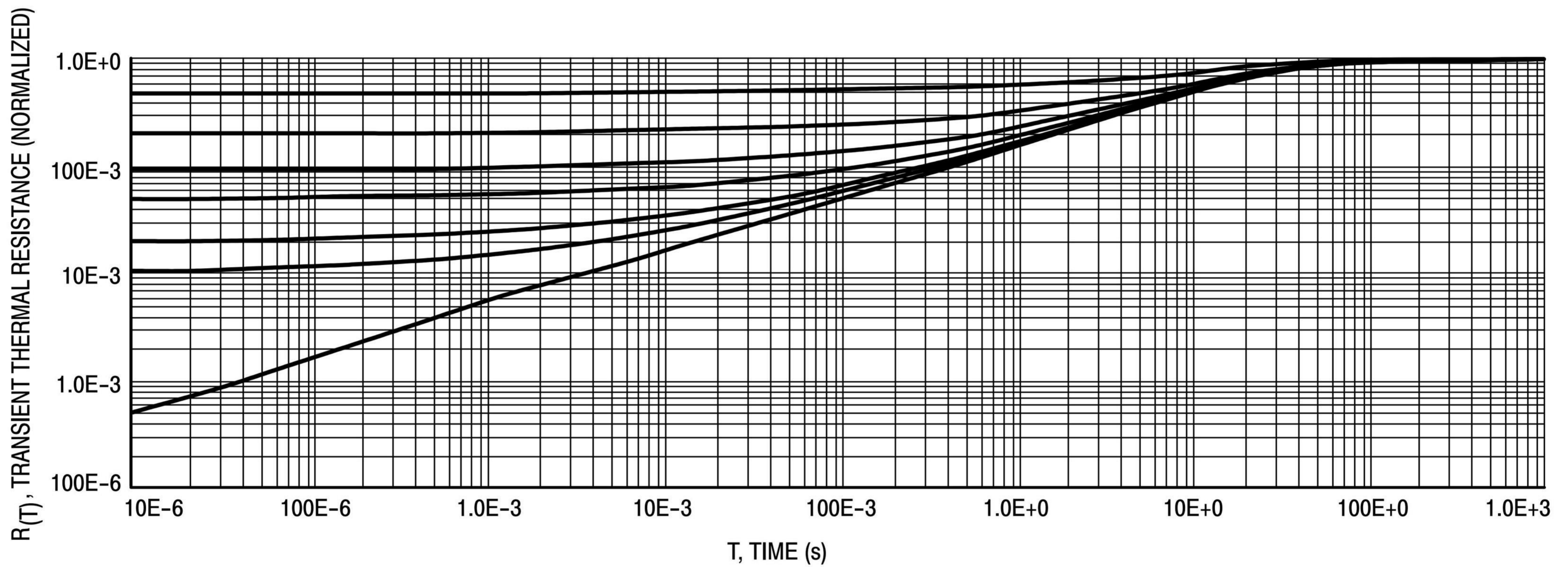
Figure 7. Thermal Response
