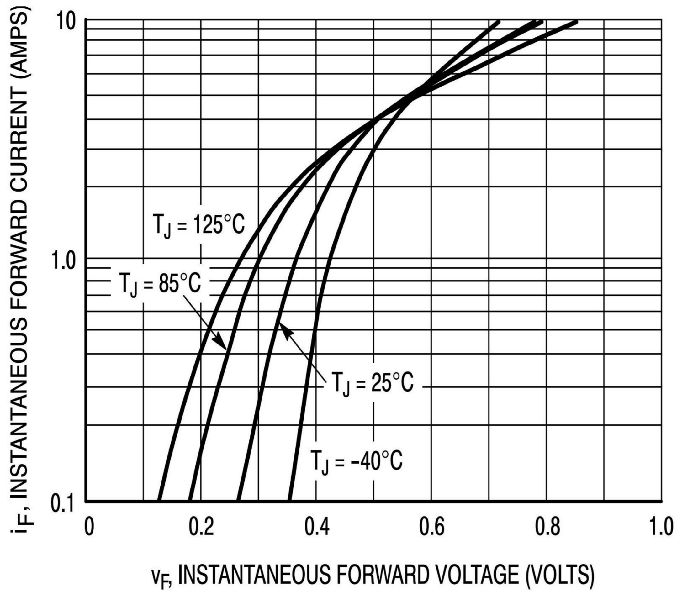
Figure 1. Typical Forward Voltage
