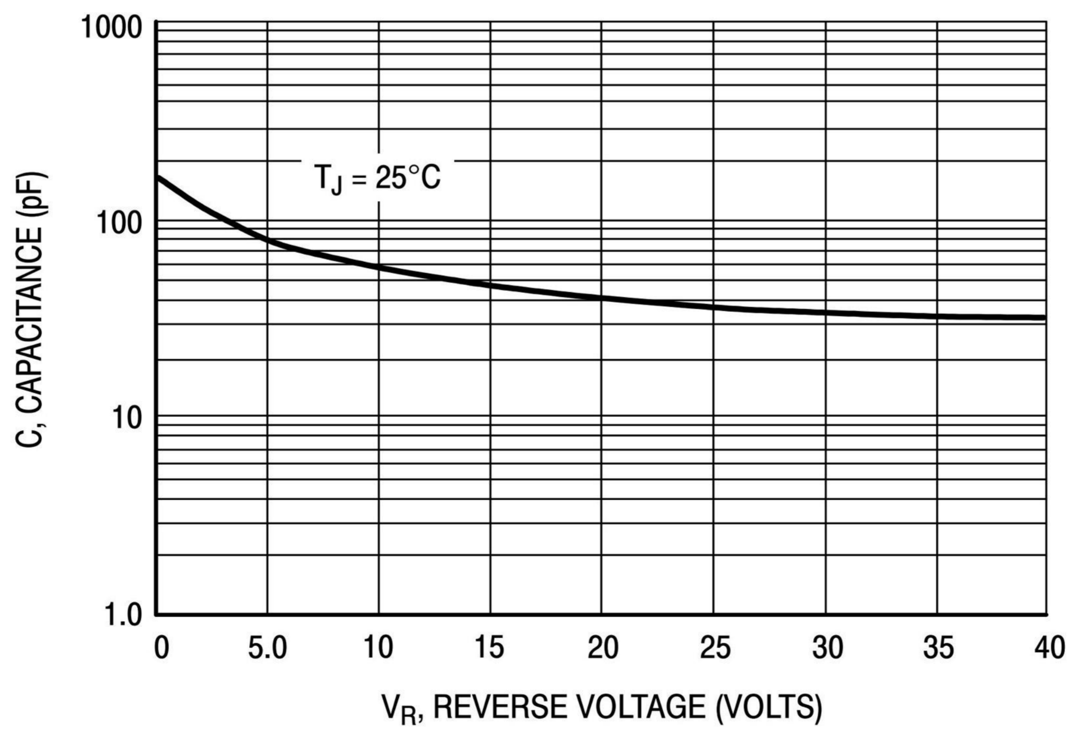
Figure 8. Capacitance
