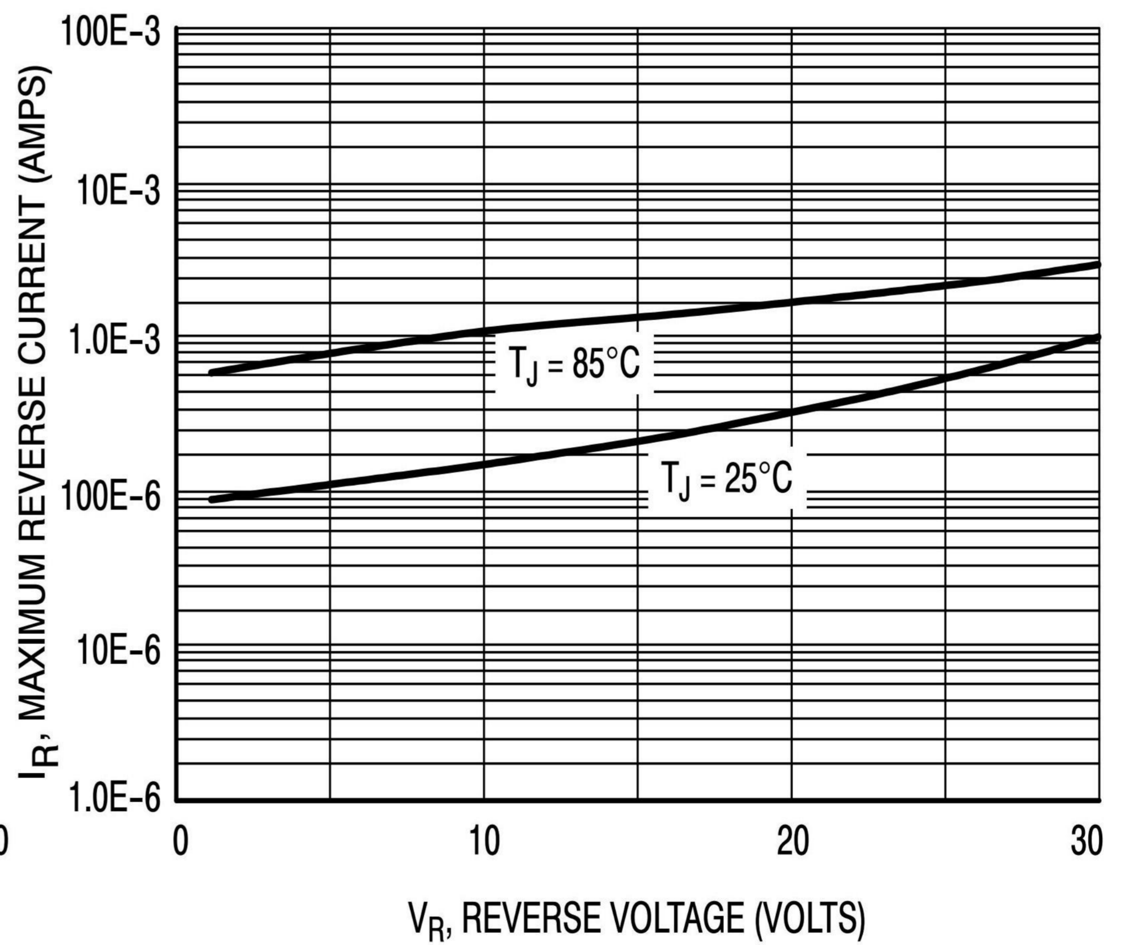
Figure 4. Maximum Reverse Current
