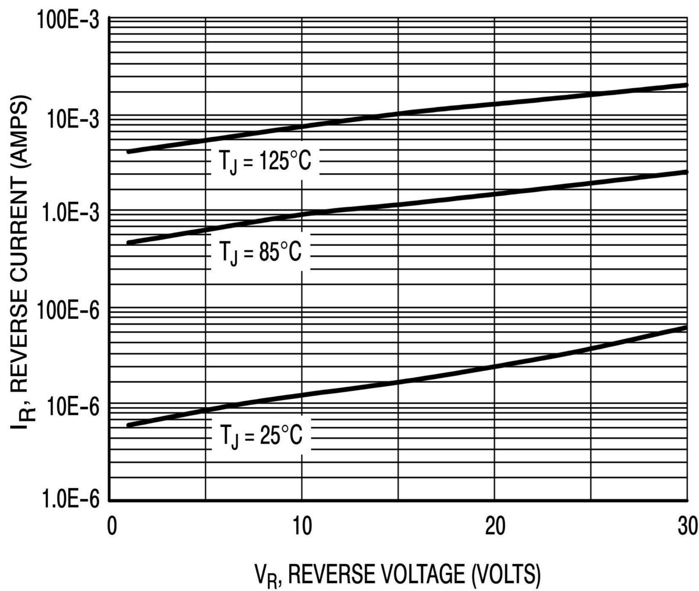
Figure 3. Typical Reverse Current
