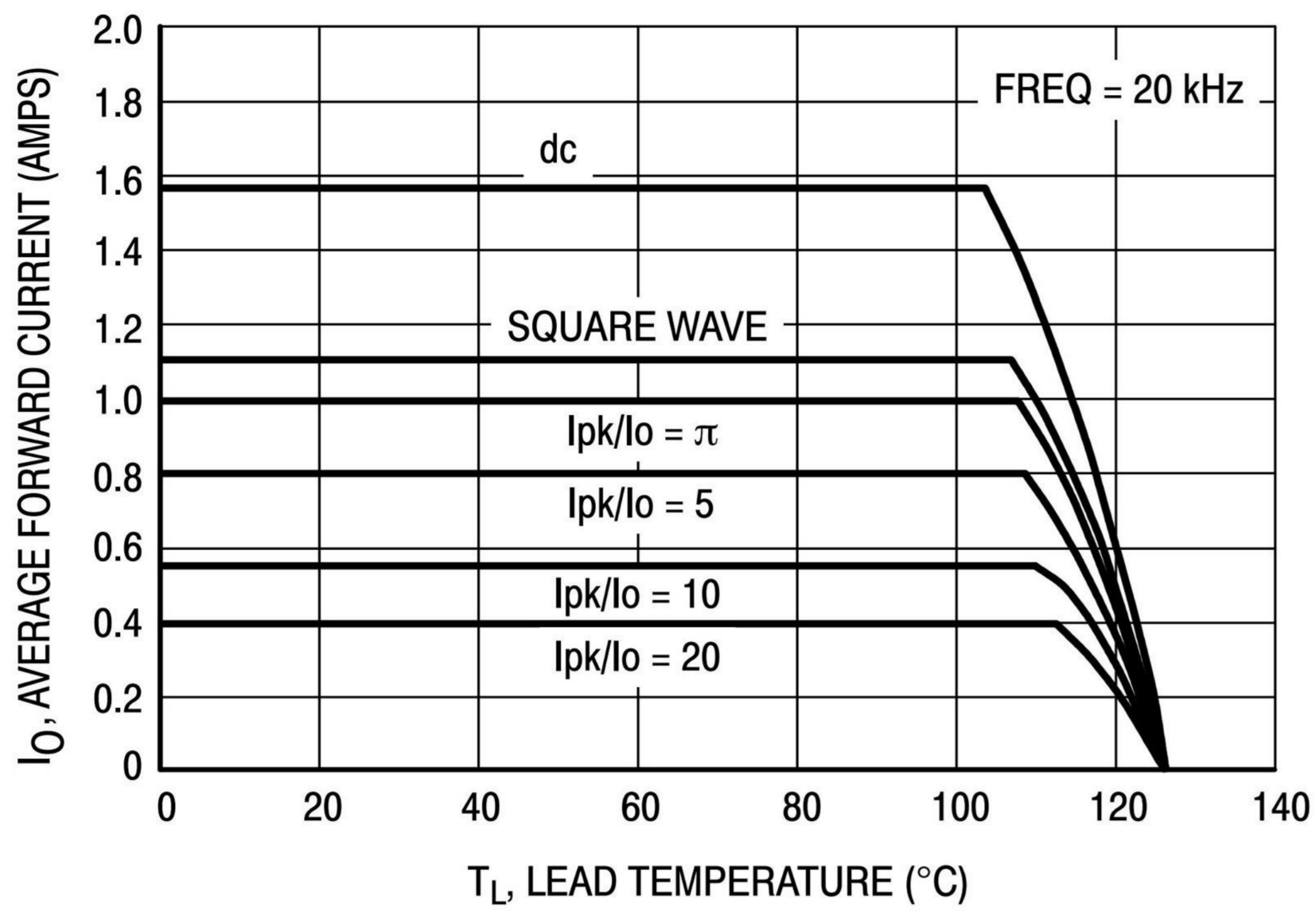
Figure 5. Current Derating
