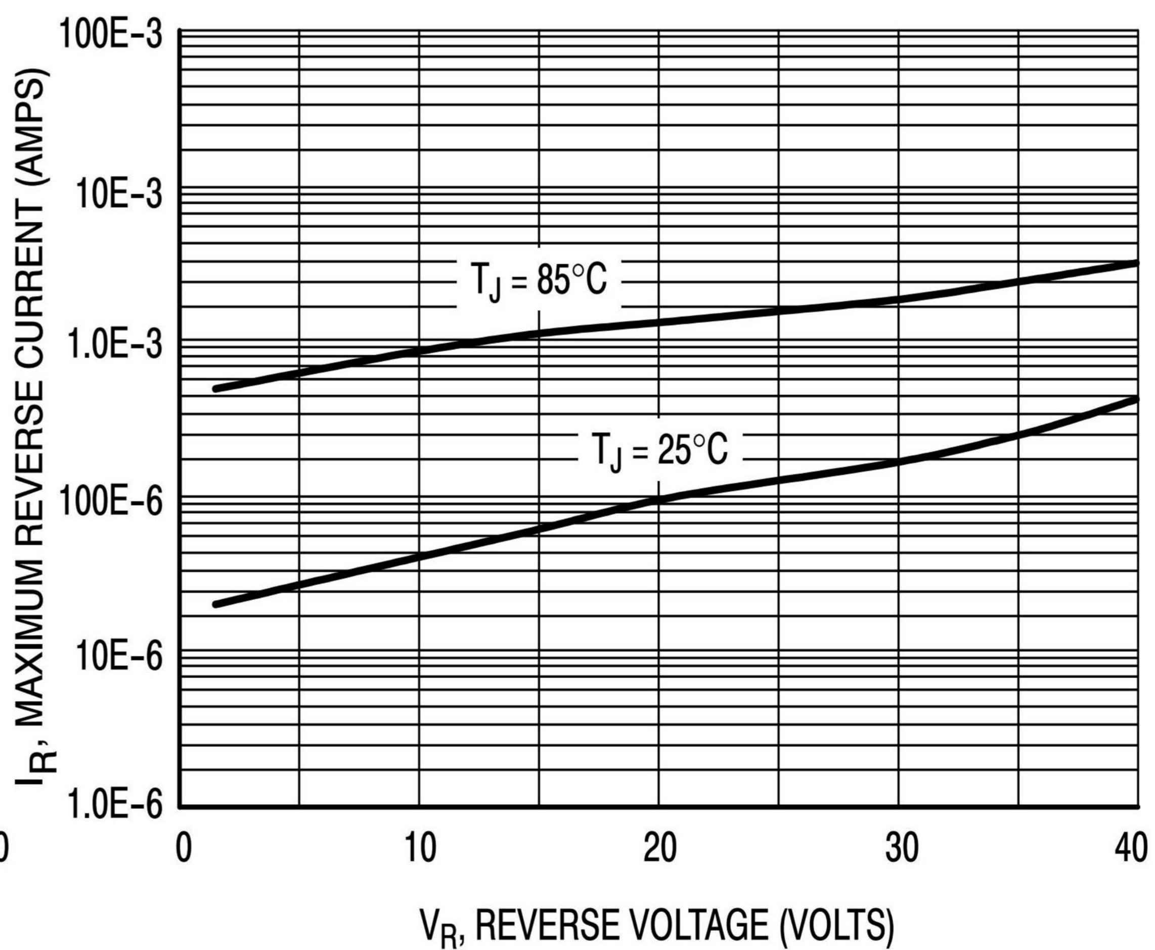
Figure 4. Maximum Reverse Current
