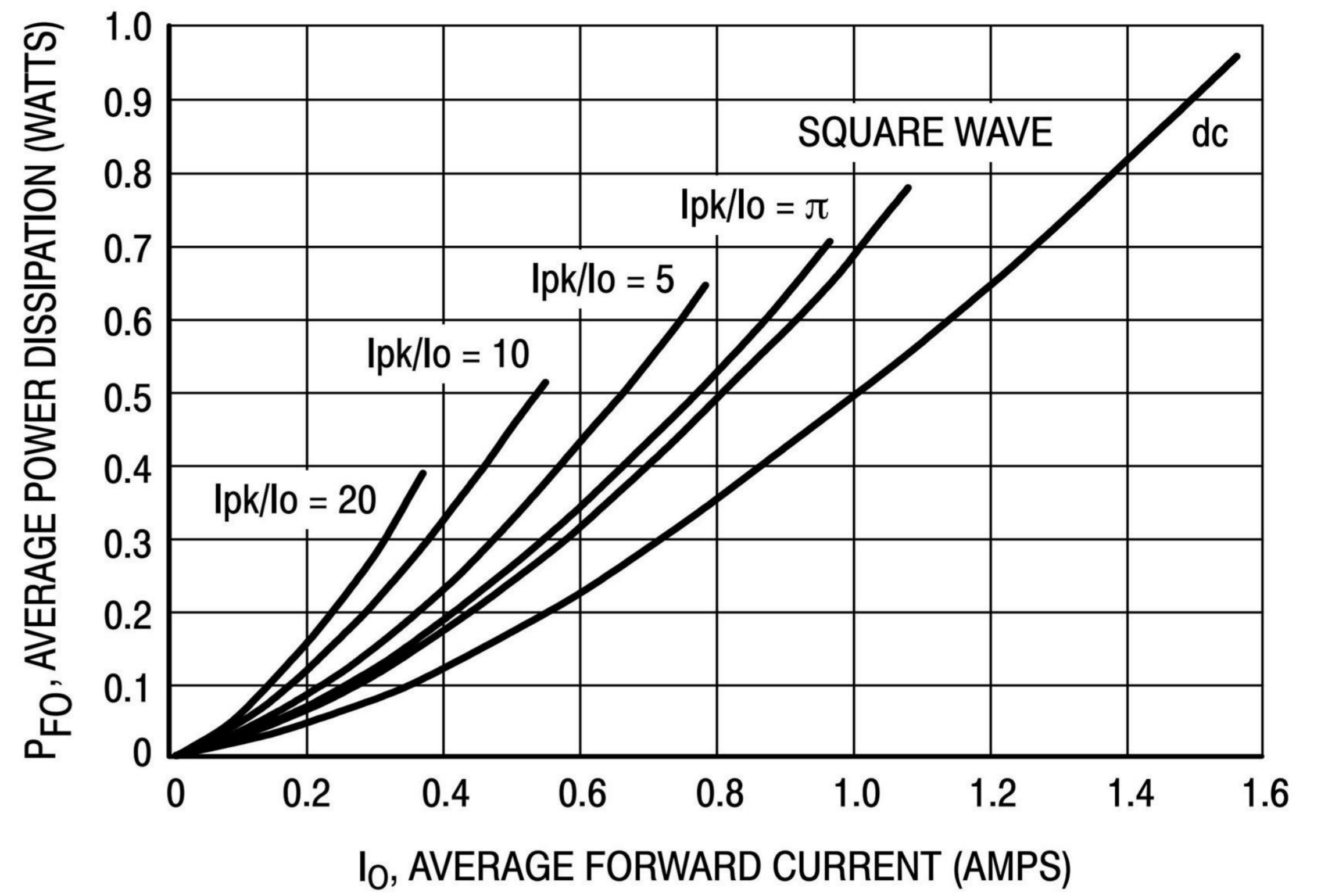
Figure 6. Forward Power Dissipation
