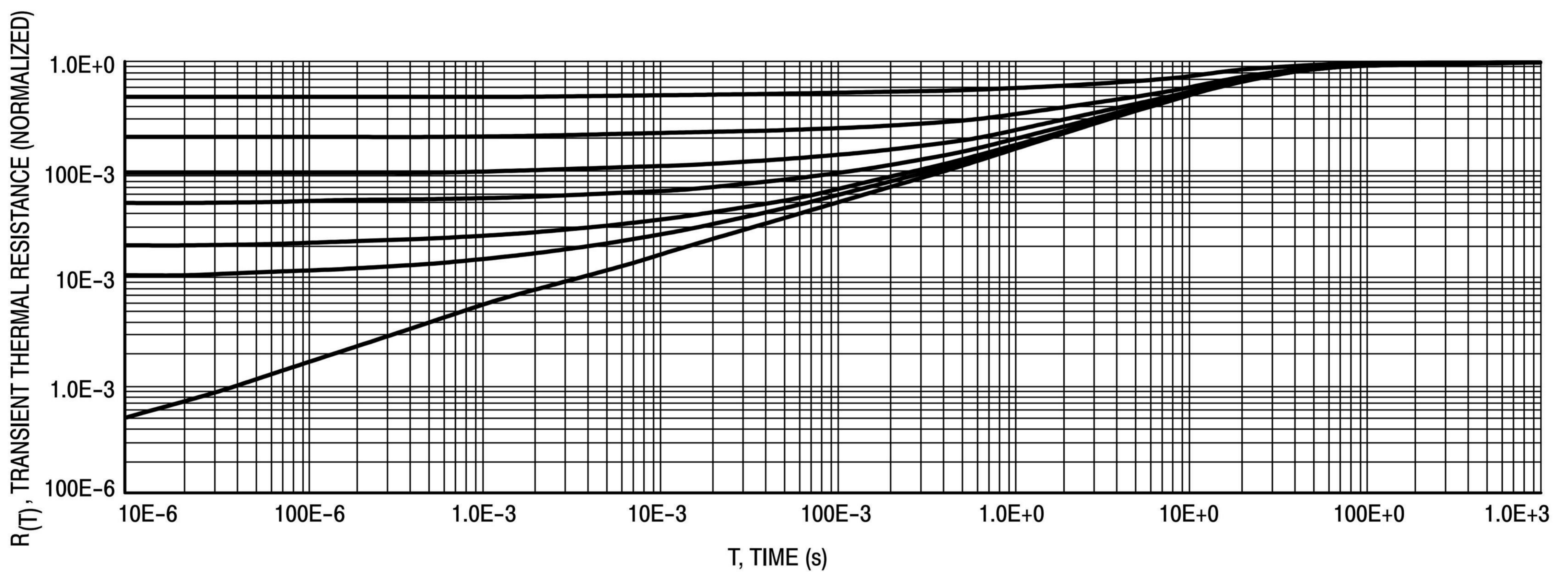
Figure 7. Thermal Response
