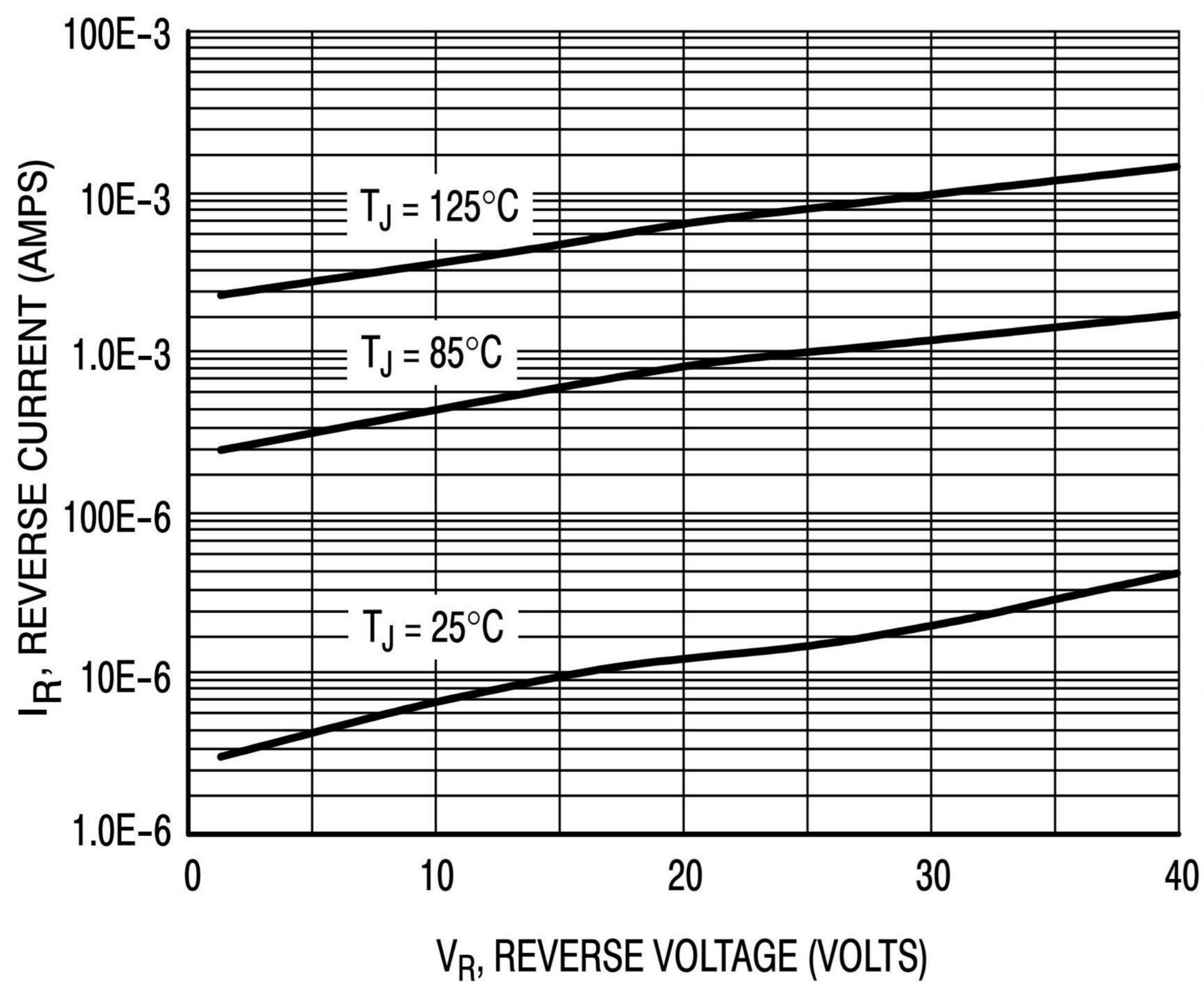
Figure 3. Typical Reverse Current
