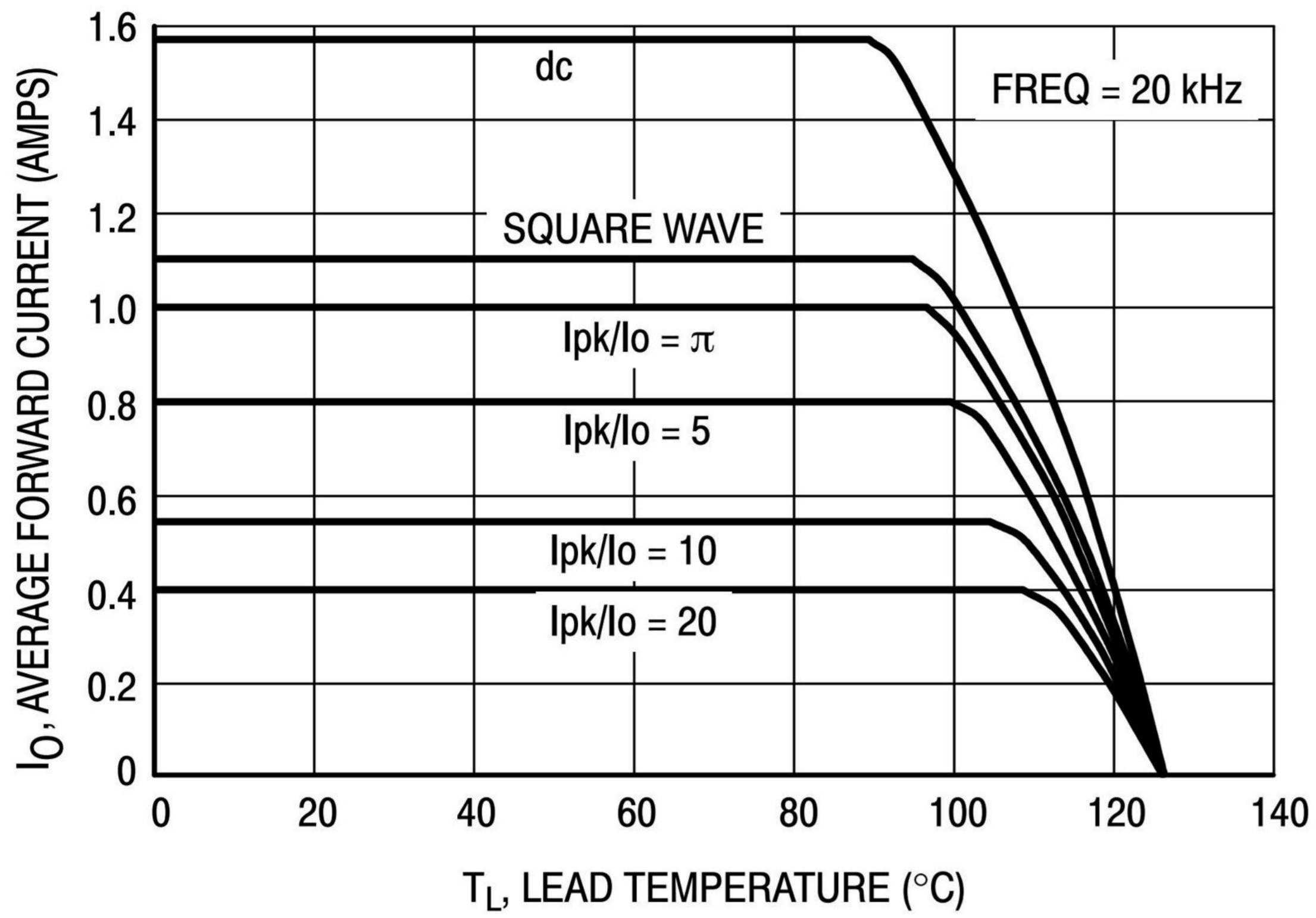
Figure 5. Current Derating
