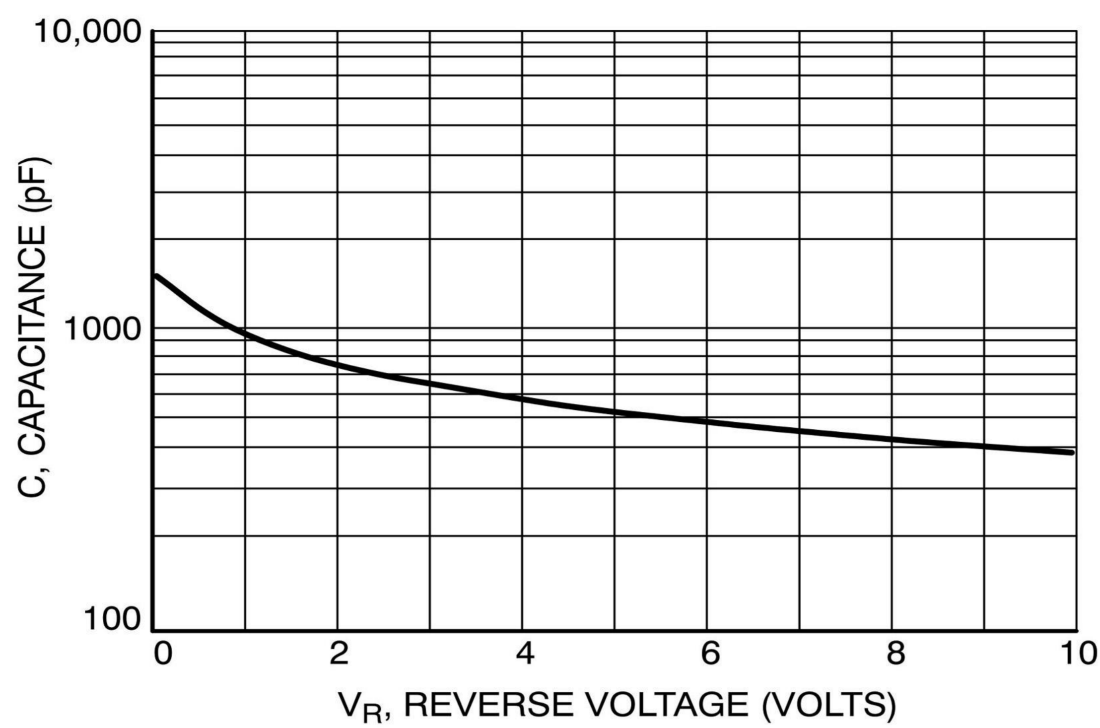
Figure 6. Typical Capacitance
