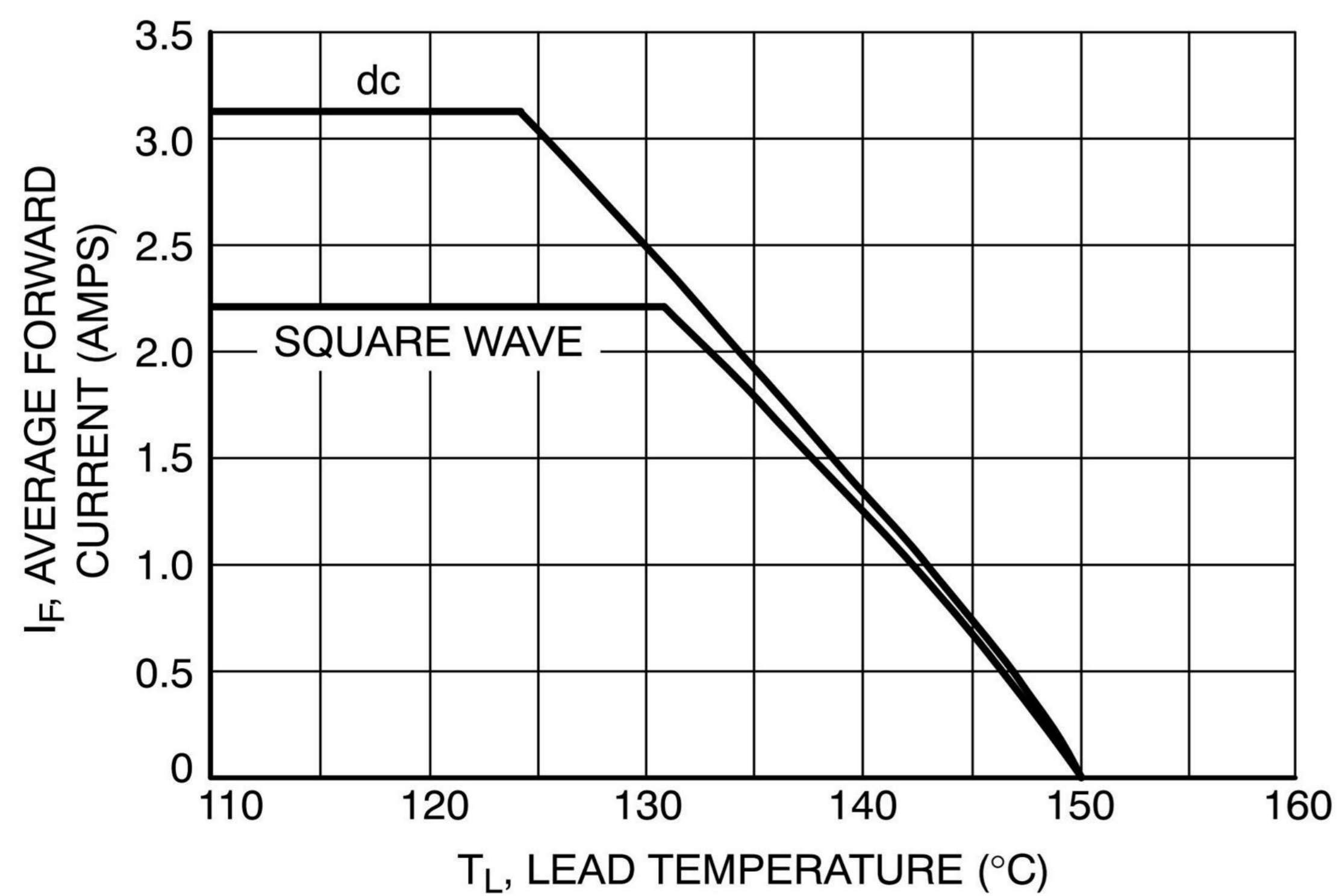
Figure 4. Current Derating - Junction to Lead
