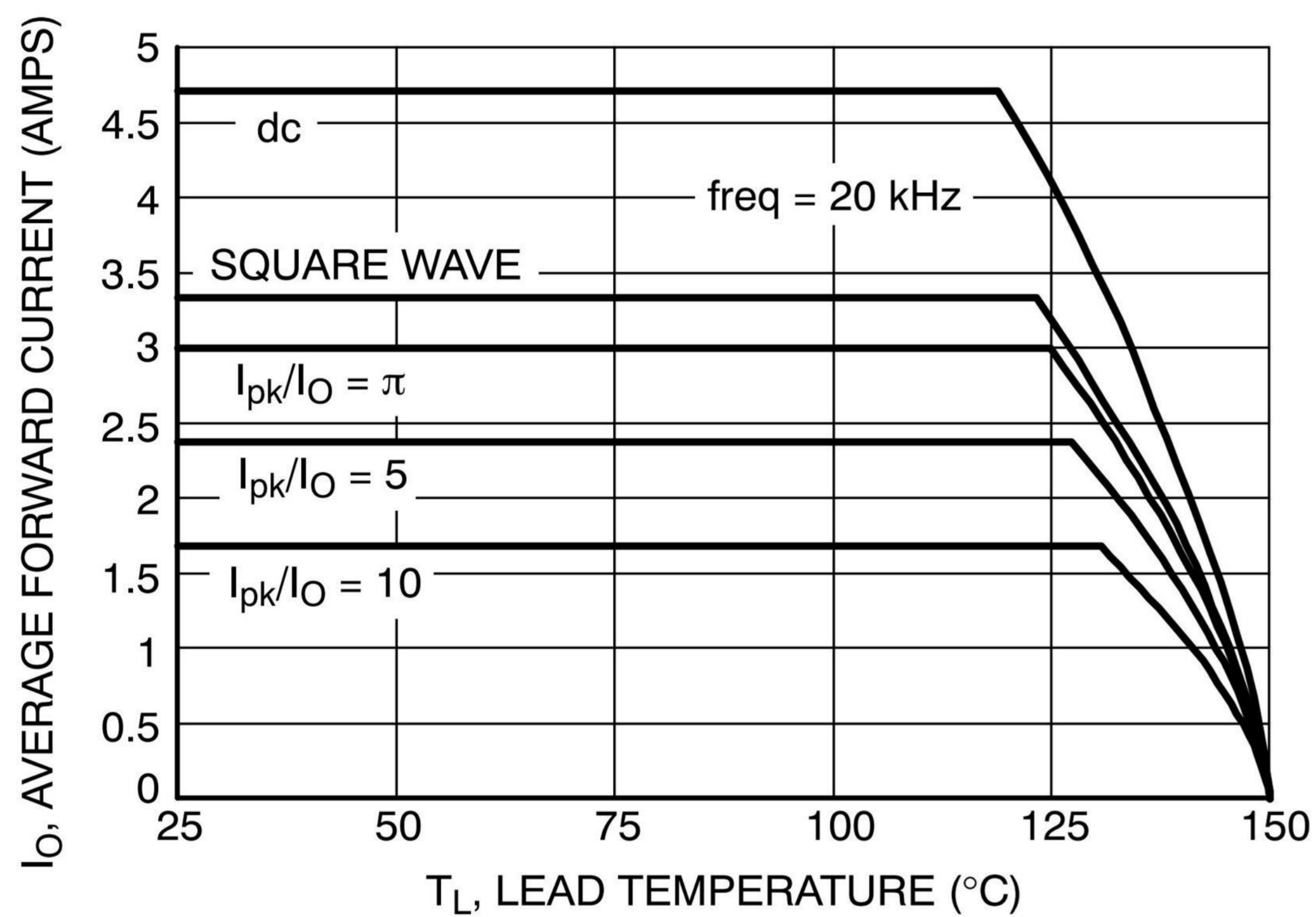
Figure 5. Current Derating
