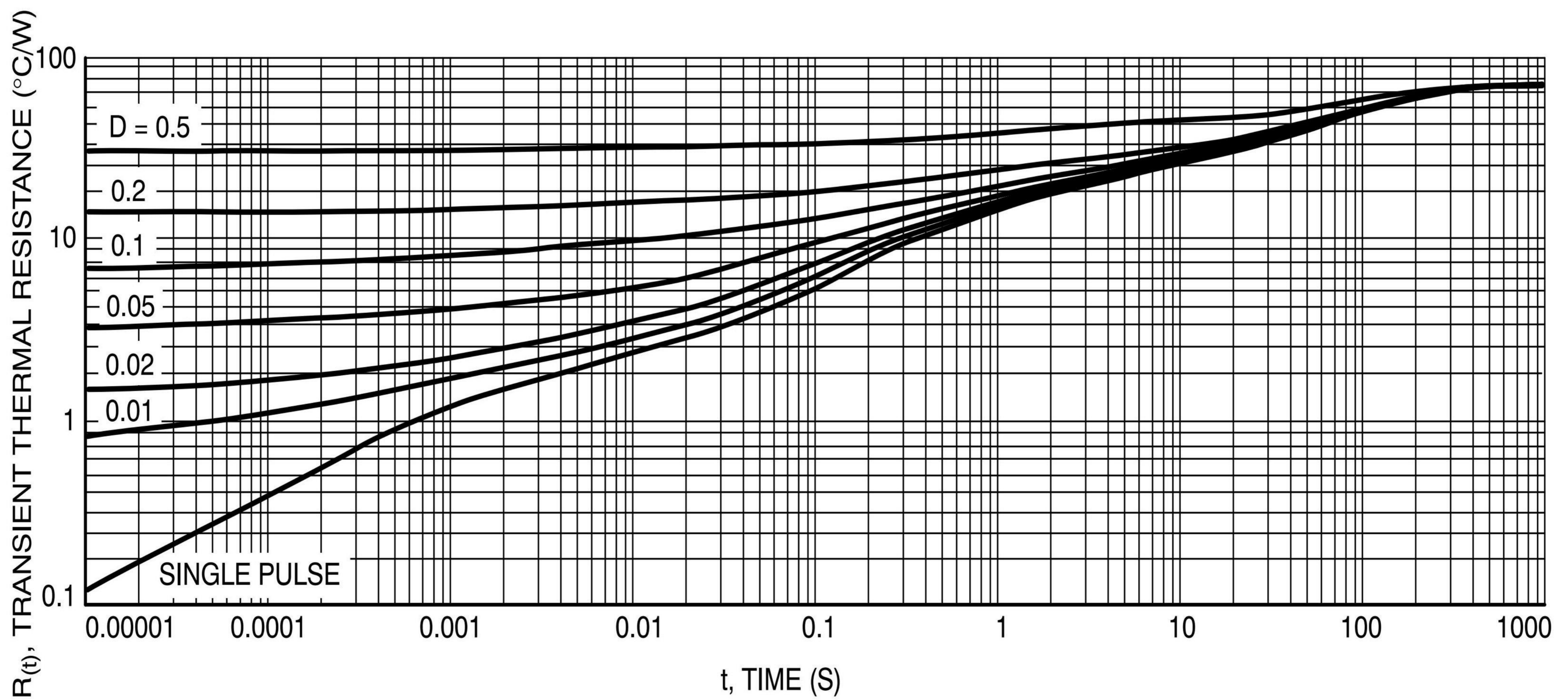
Figure 10. Thermal Response, Junction to Ambient (1 inch pad)
