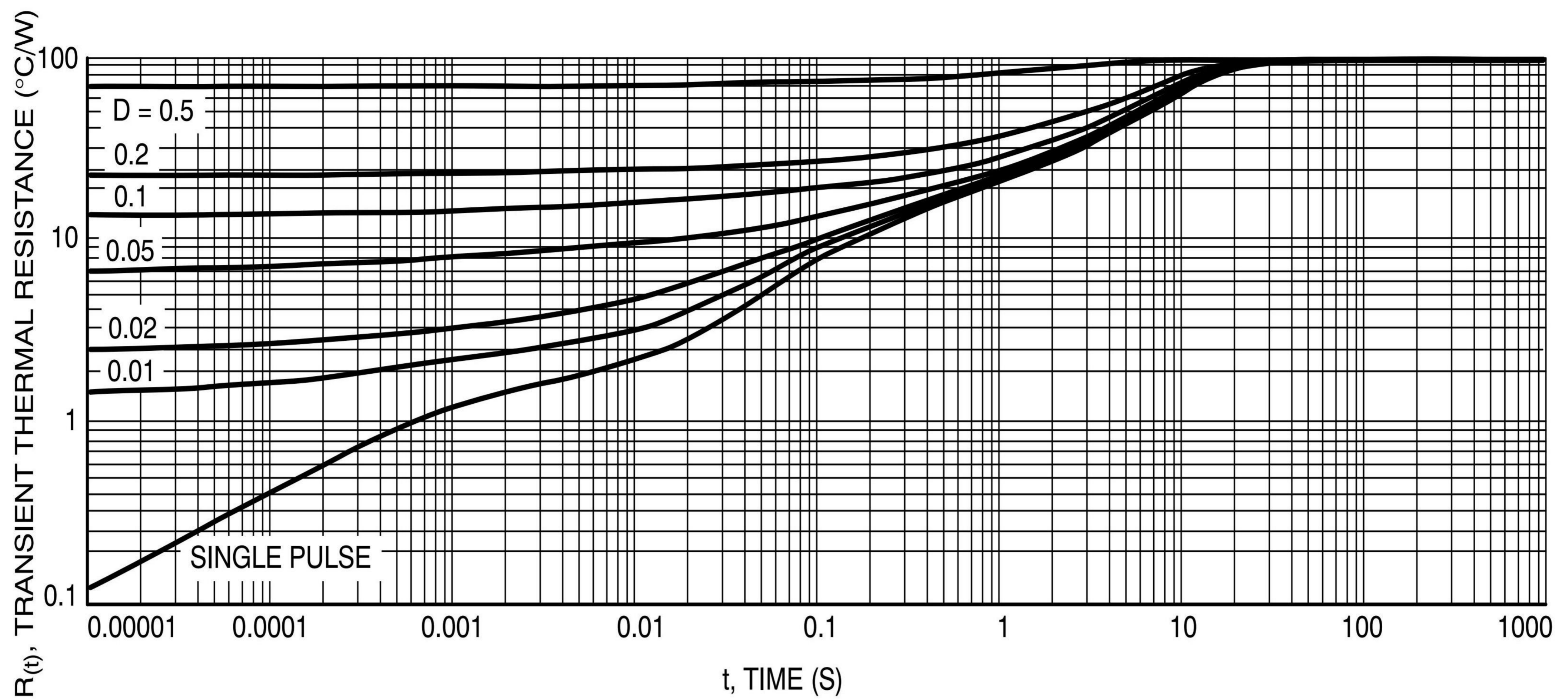
Figure 9. Thermal Response, Junction-to-Ambient (min pad)
