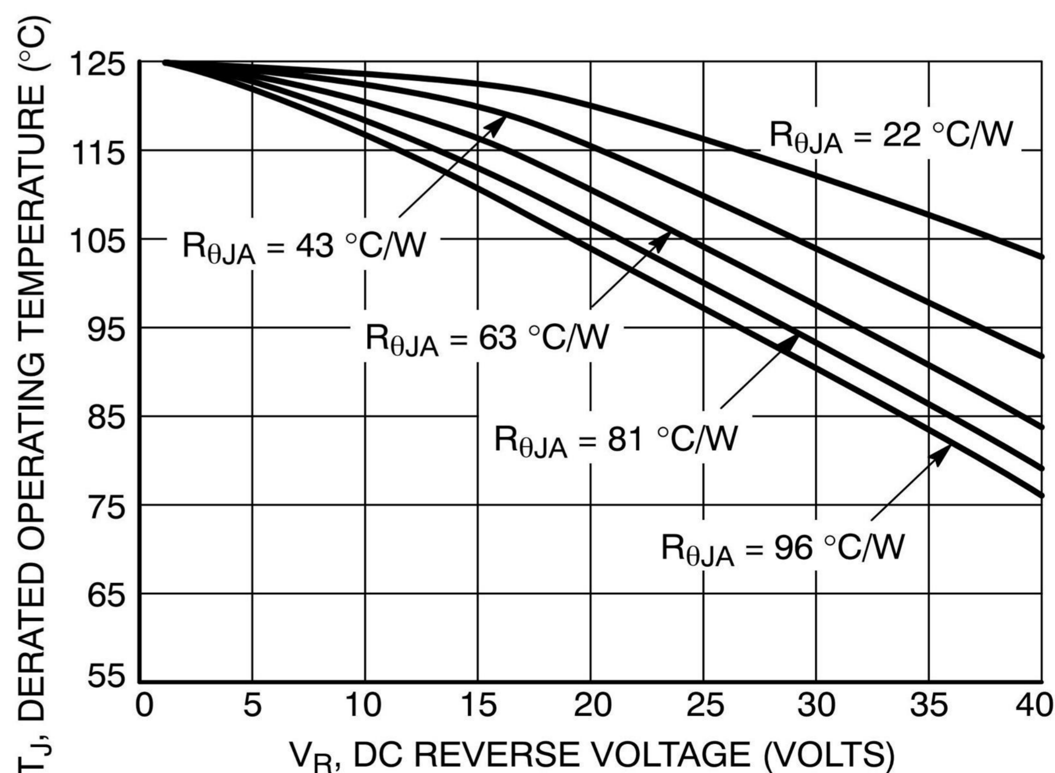
Figure 8. Typical Operating Temperature Derating
