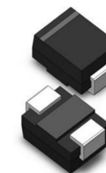
SMA CASE 403D STYLE 1
