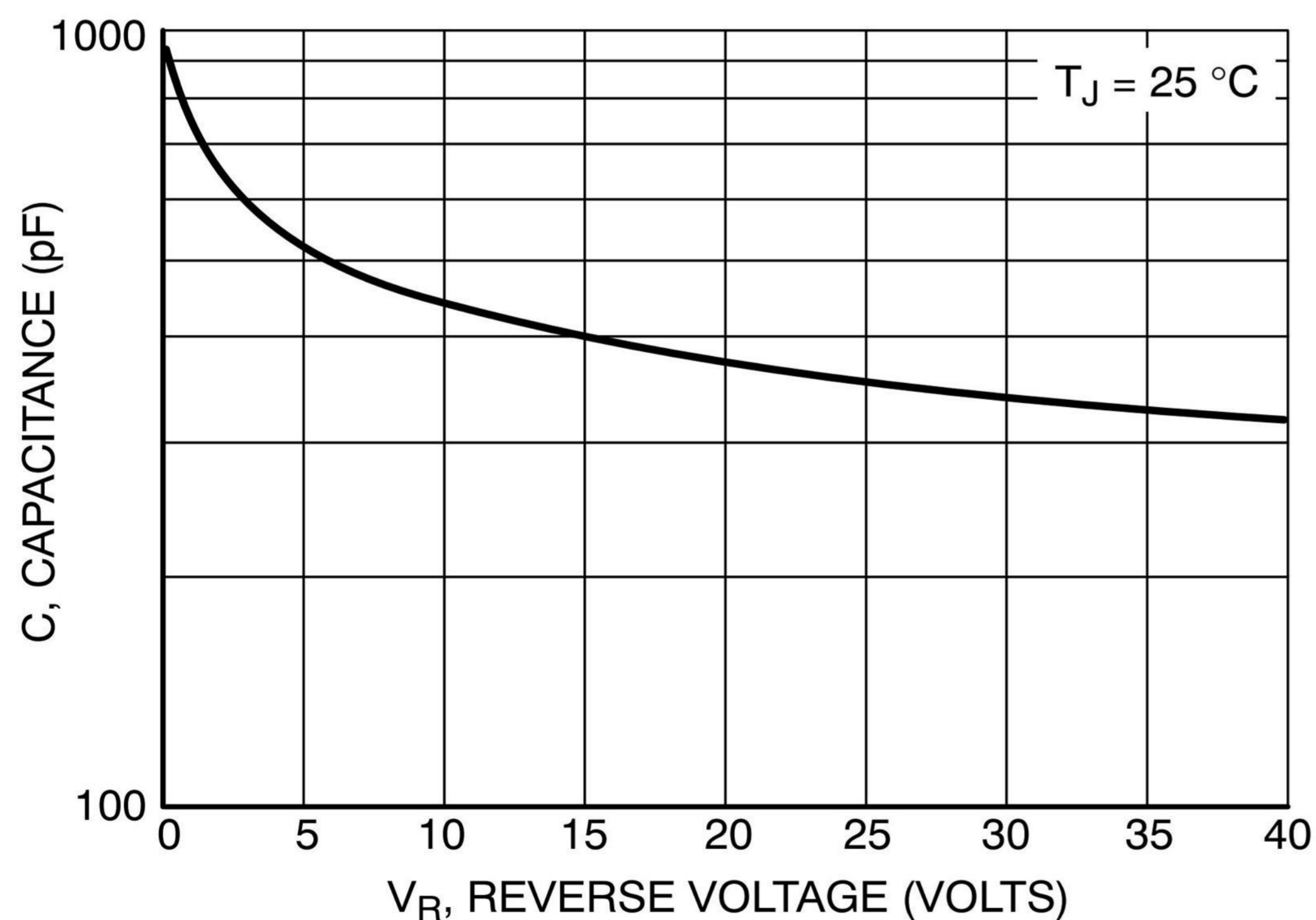
Figure 7. Capacitance
