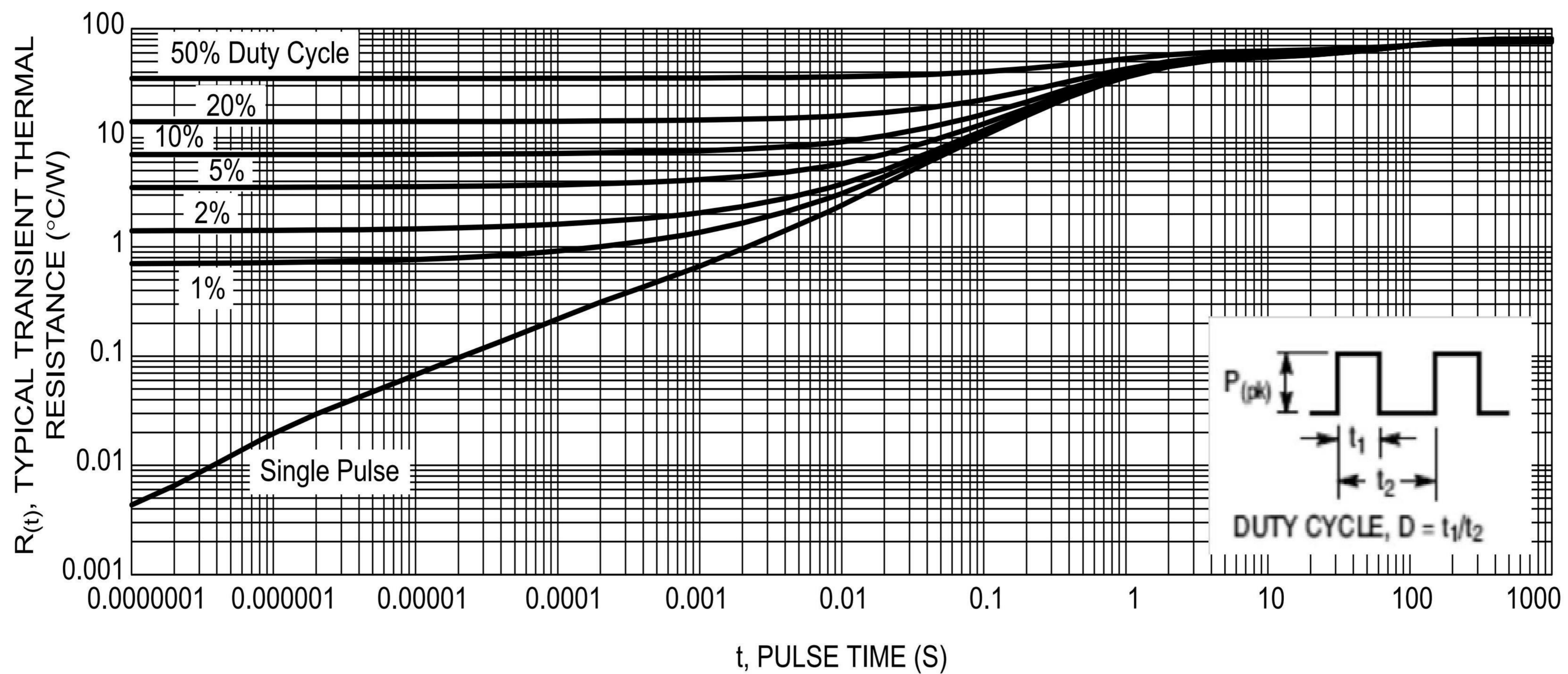
Figure 6. Typical Transient Thermal Response, Junction-to-Ambient
