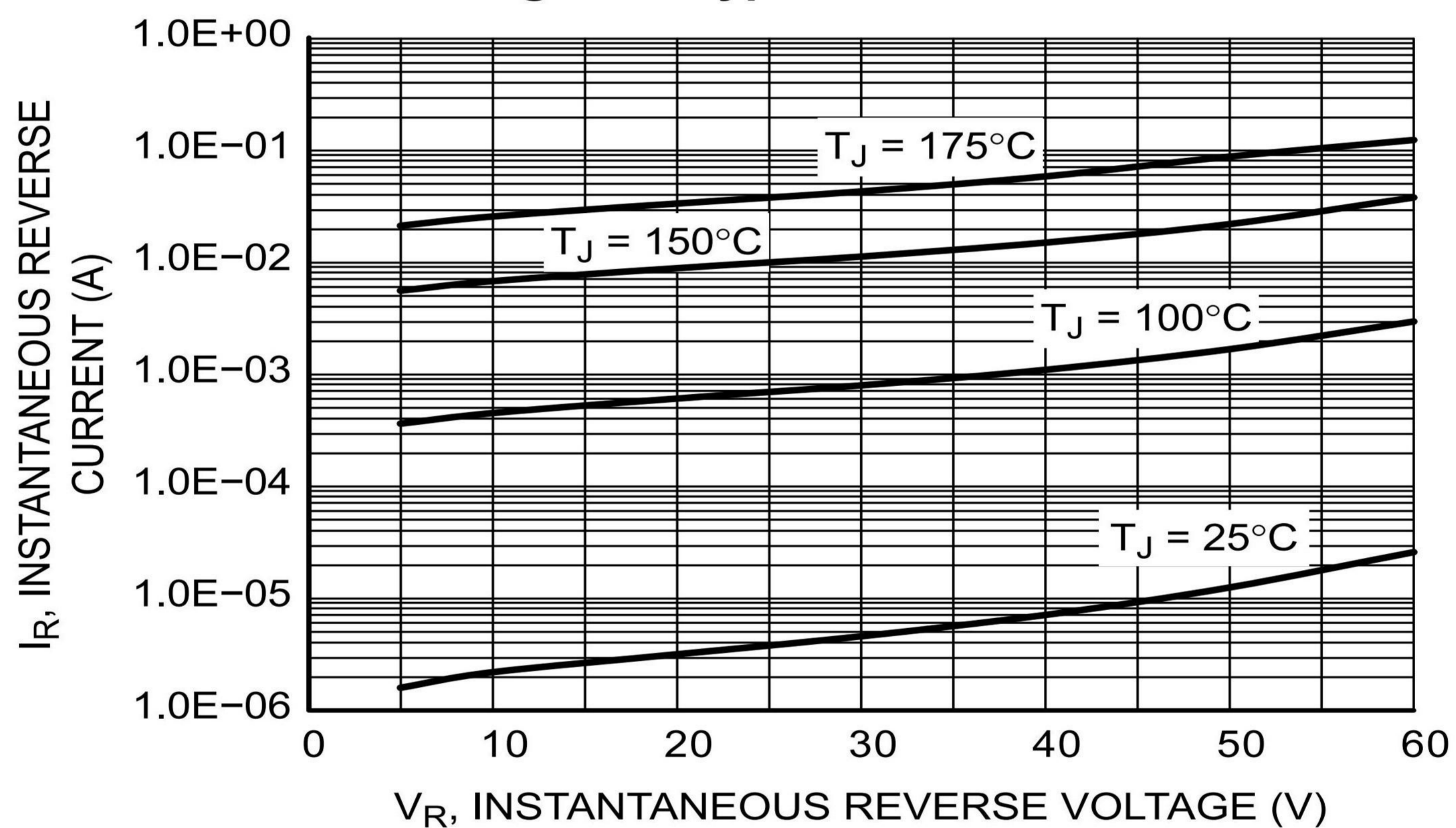
Figure 4. Maximum Reverse Current
