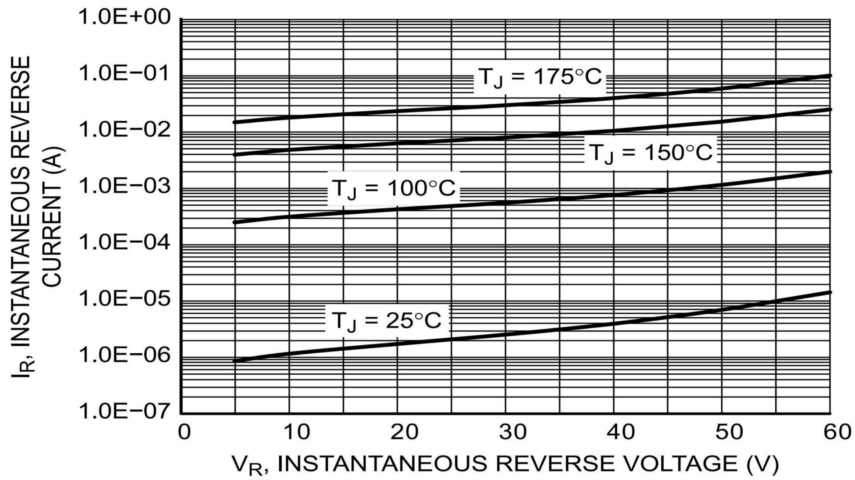
Figure 3. Typical Reverse Current
