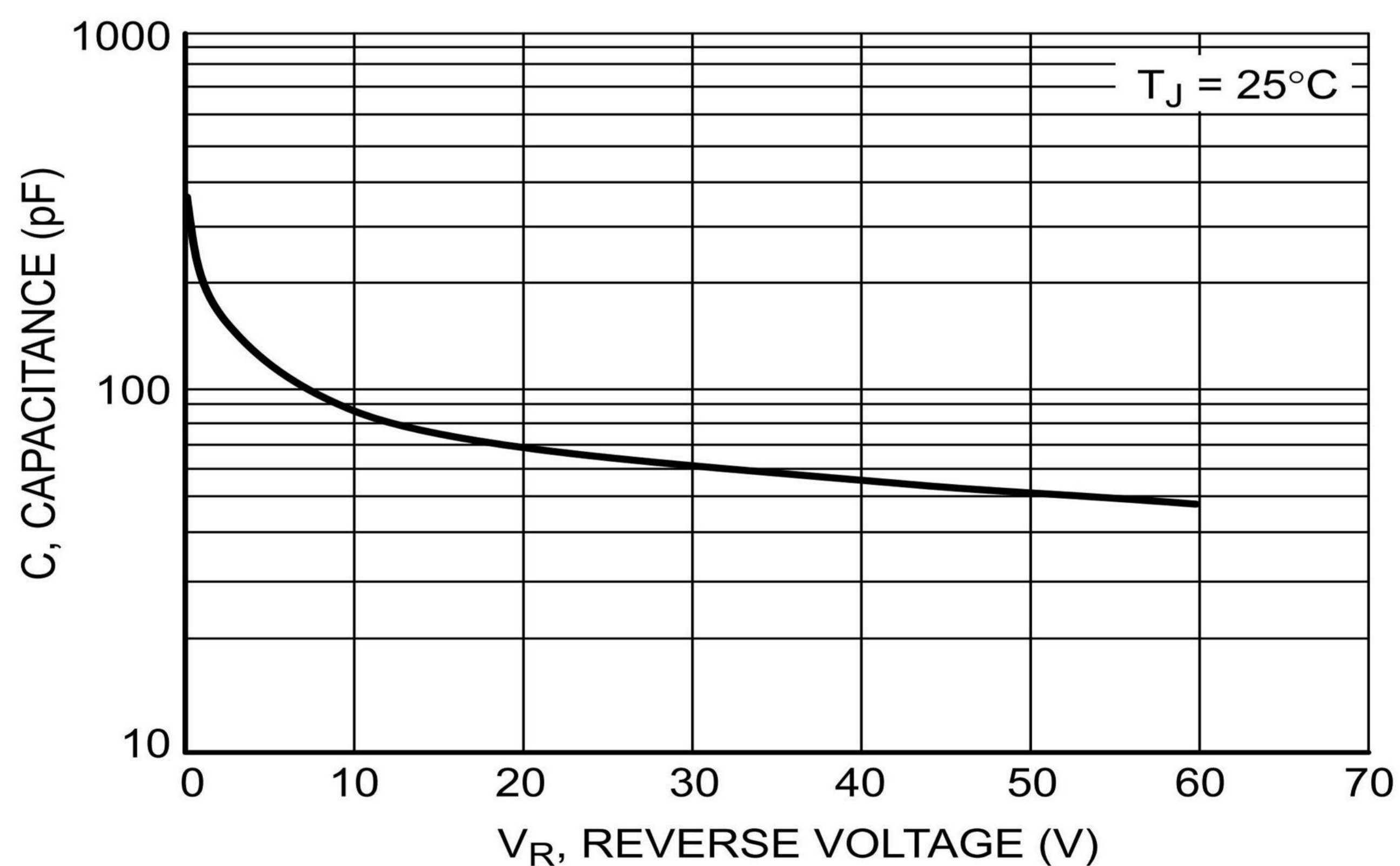
Figure 5. Typical Capacitance
