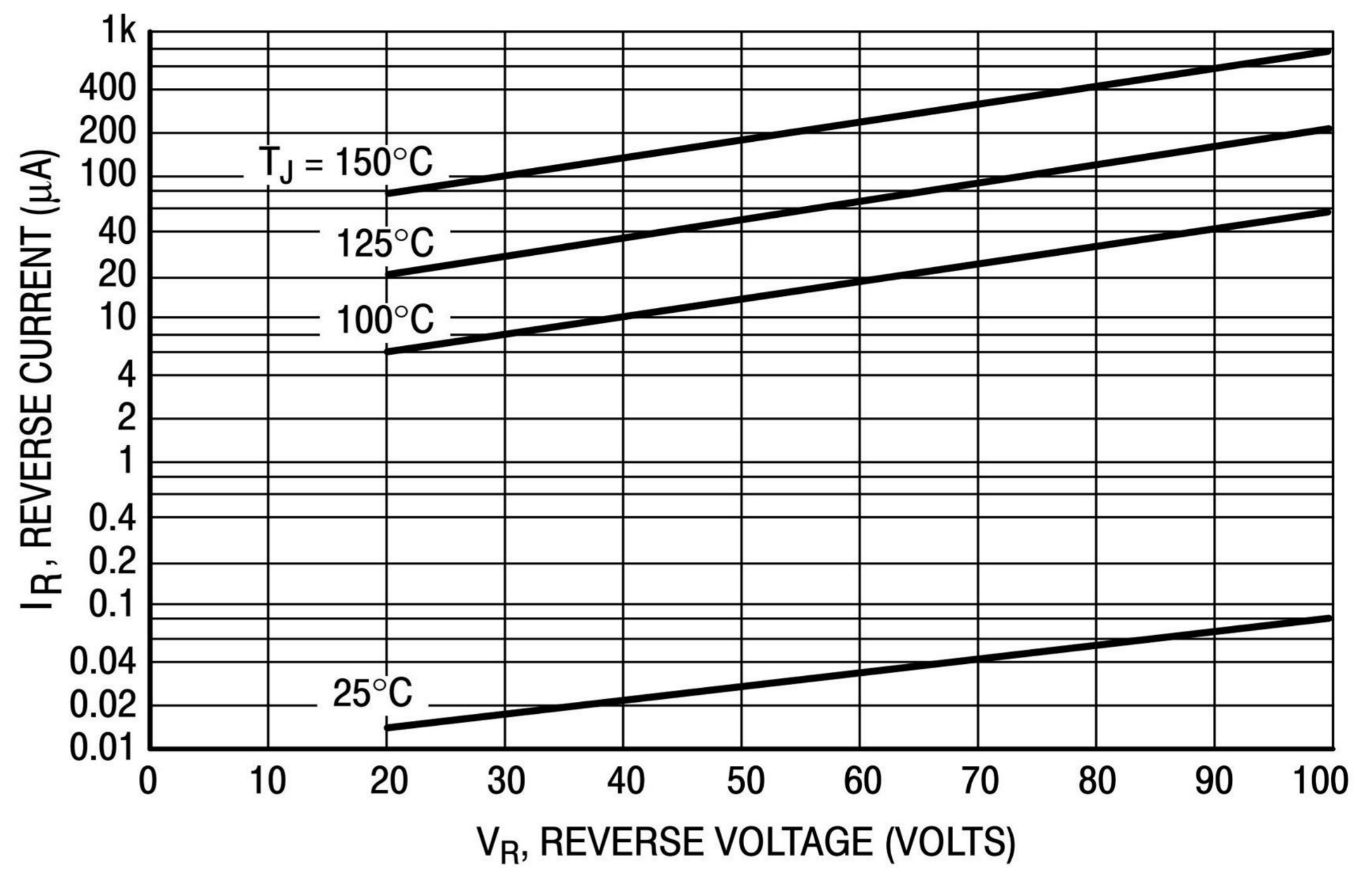
Figure 2. Typical Reverse Current*
