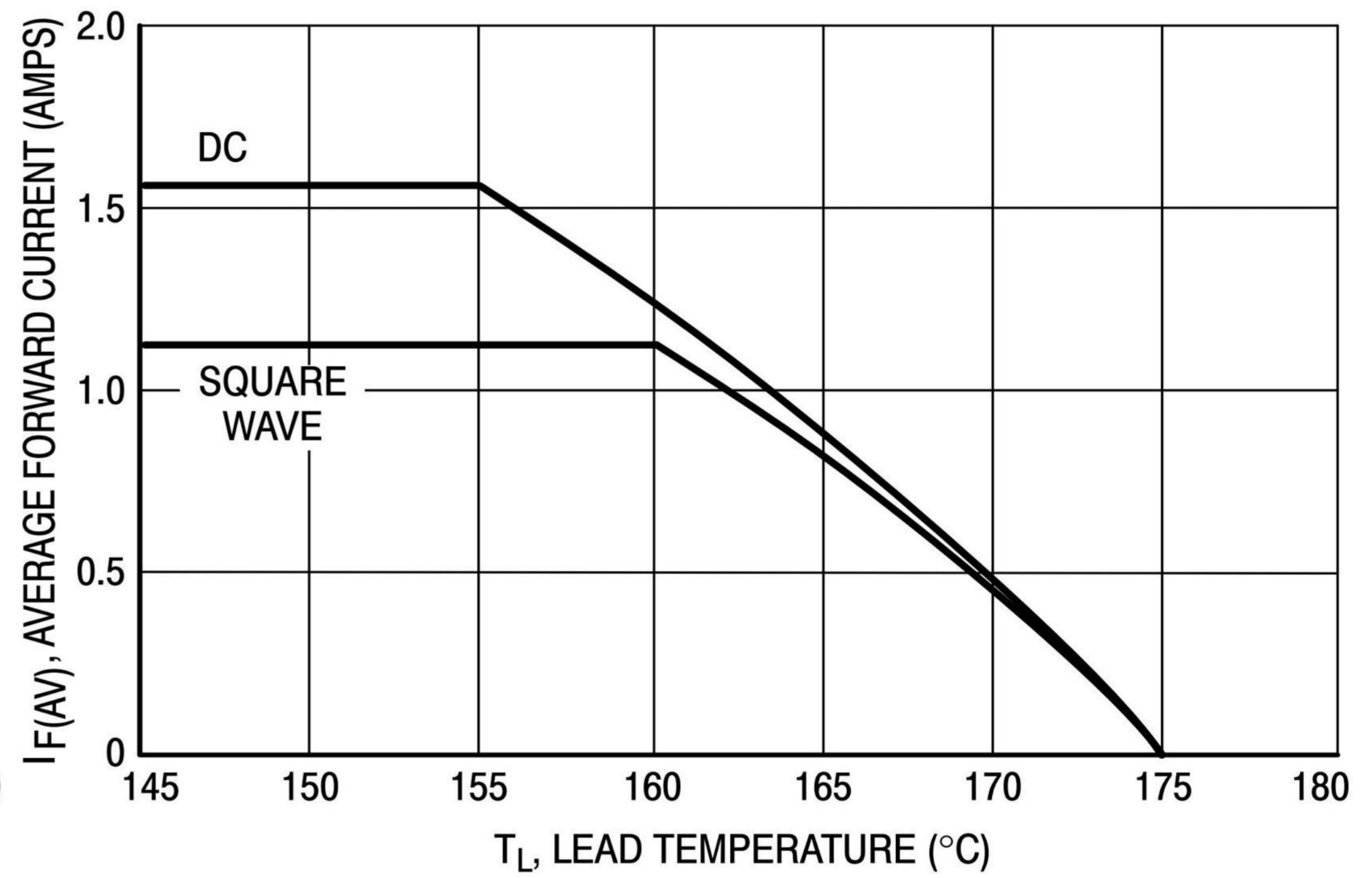
Figure 4. Current Derating, Lead
