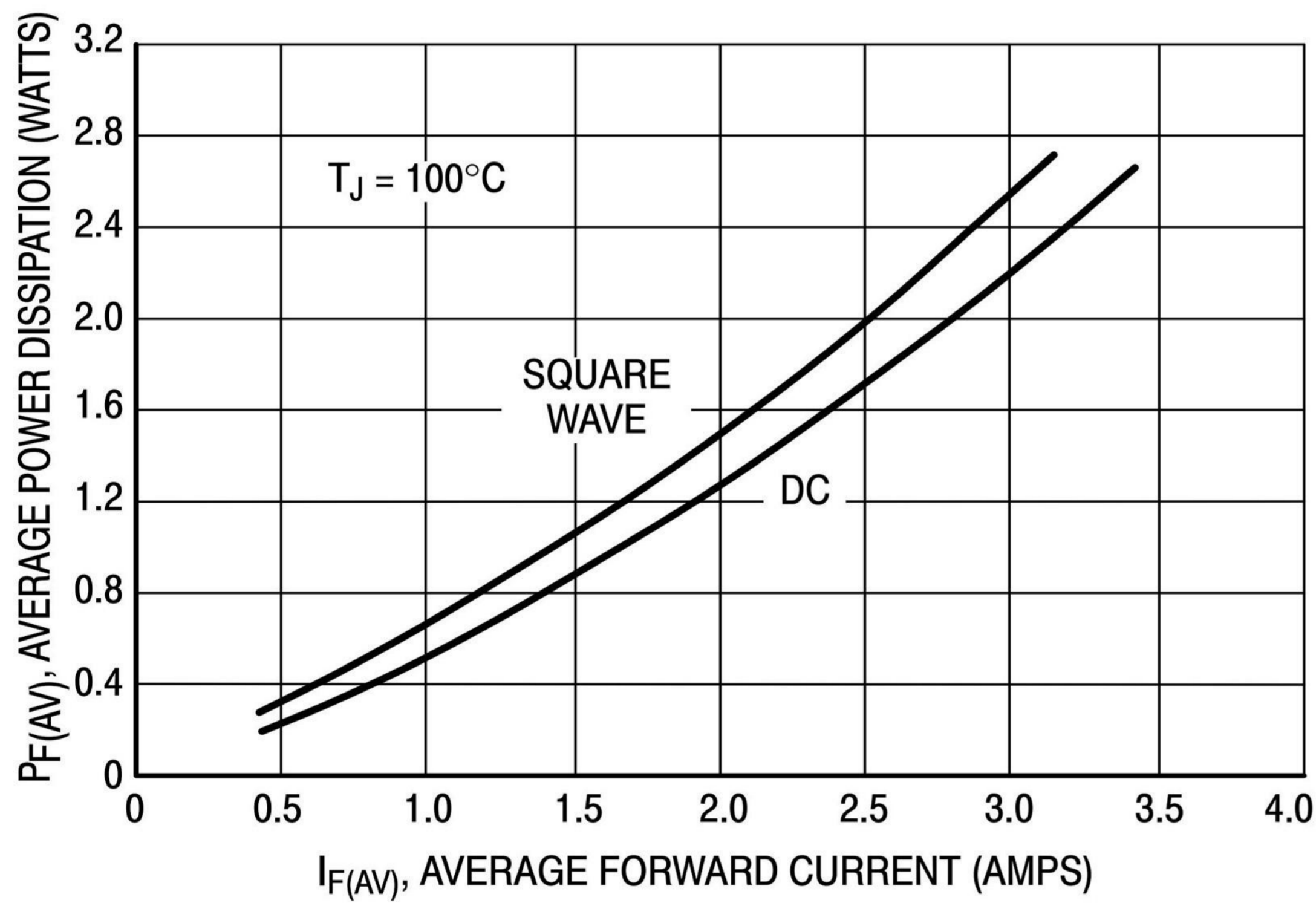
Figure 3. Power Dissipation
