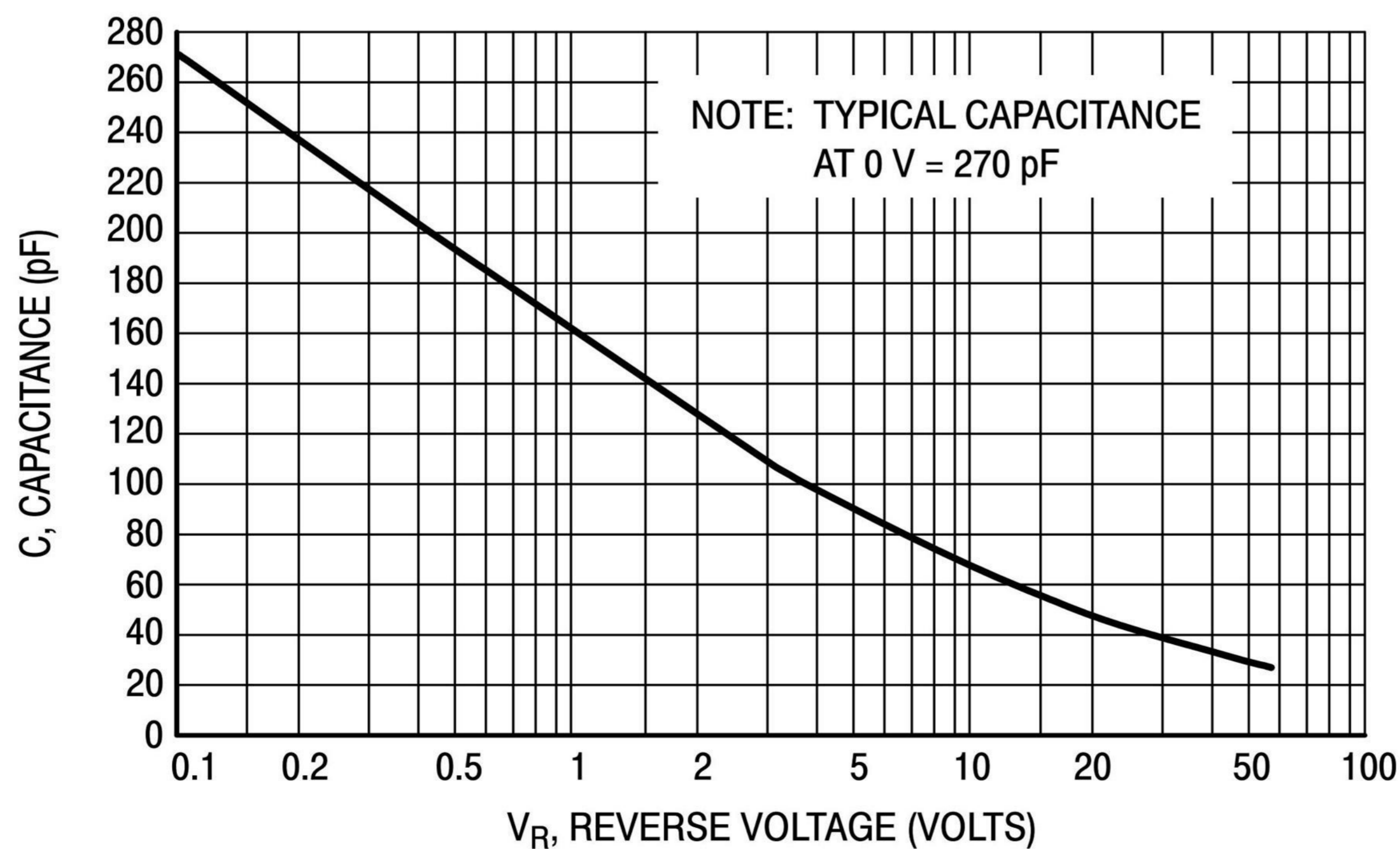
Figure 5. Typical Capacitance
