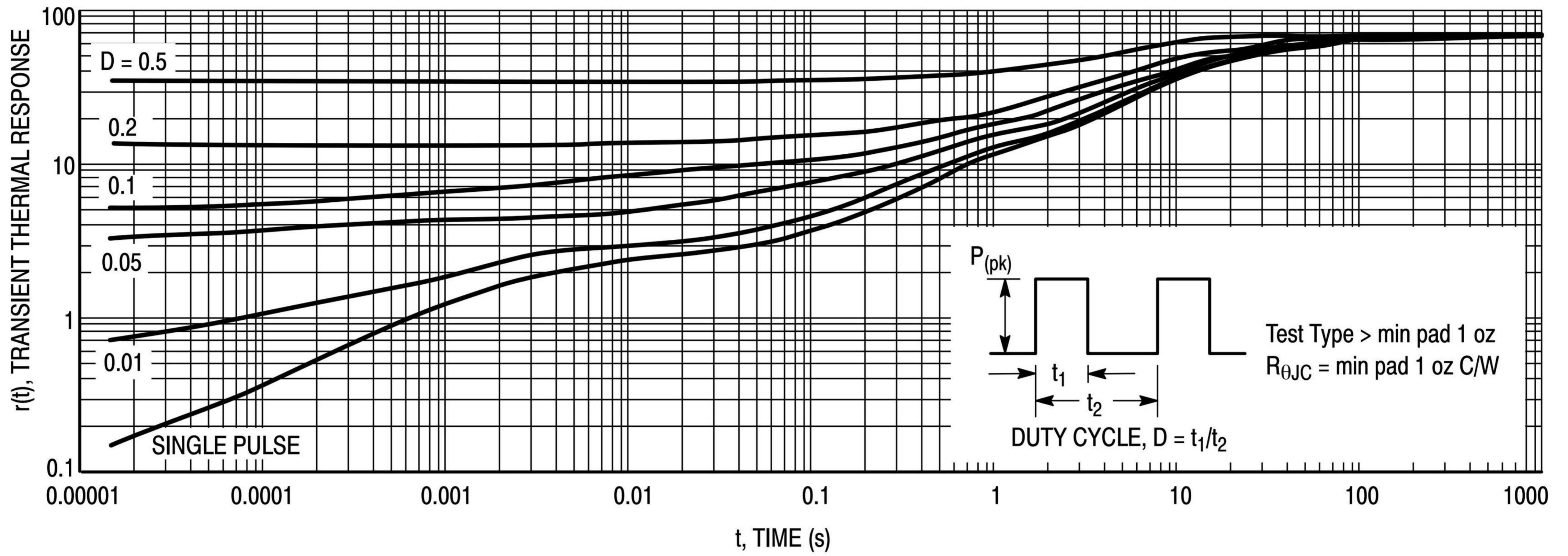
Figure 8. Thermal Response, Junction-to-Ambient, SMC Package
