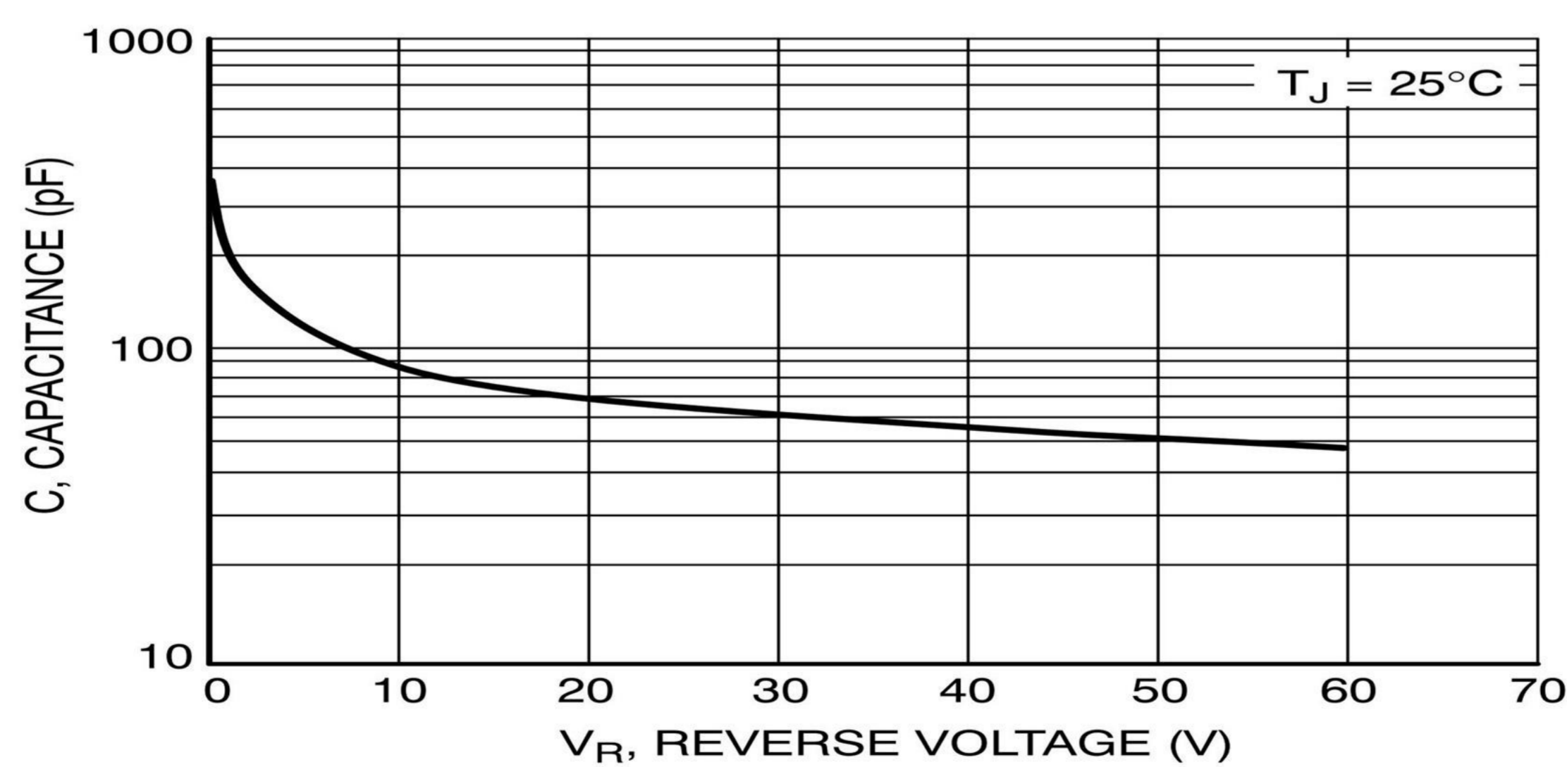
Figure 7. Typical Capacitance
