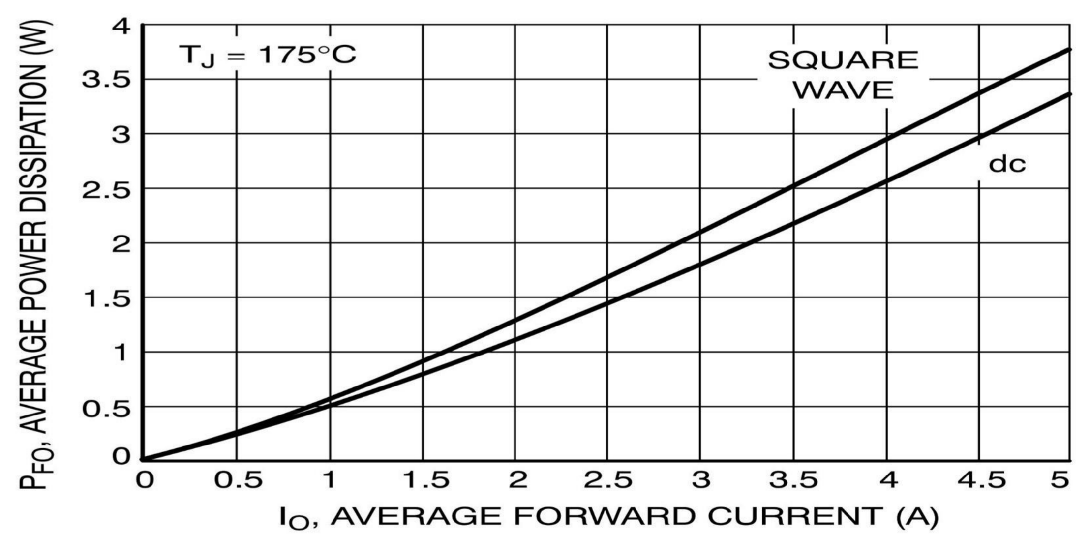
Figure 6. Forward Power Dissipation
