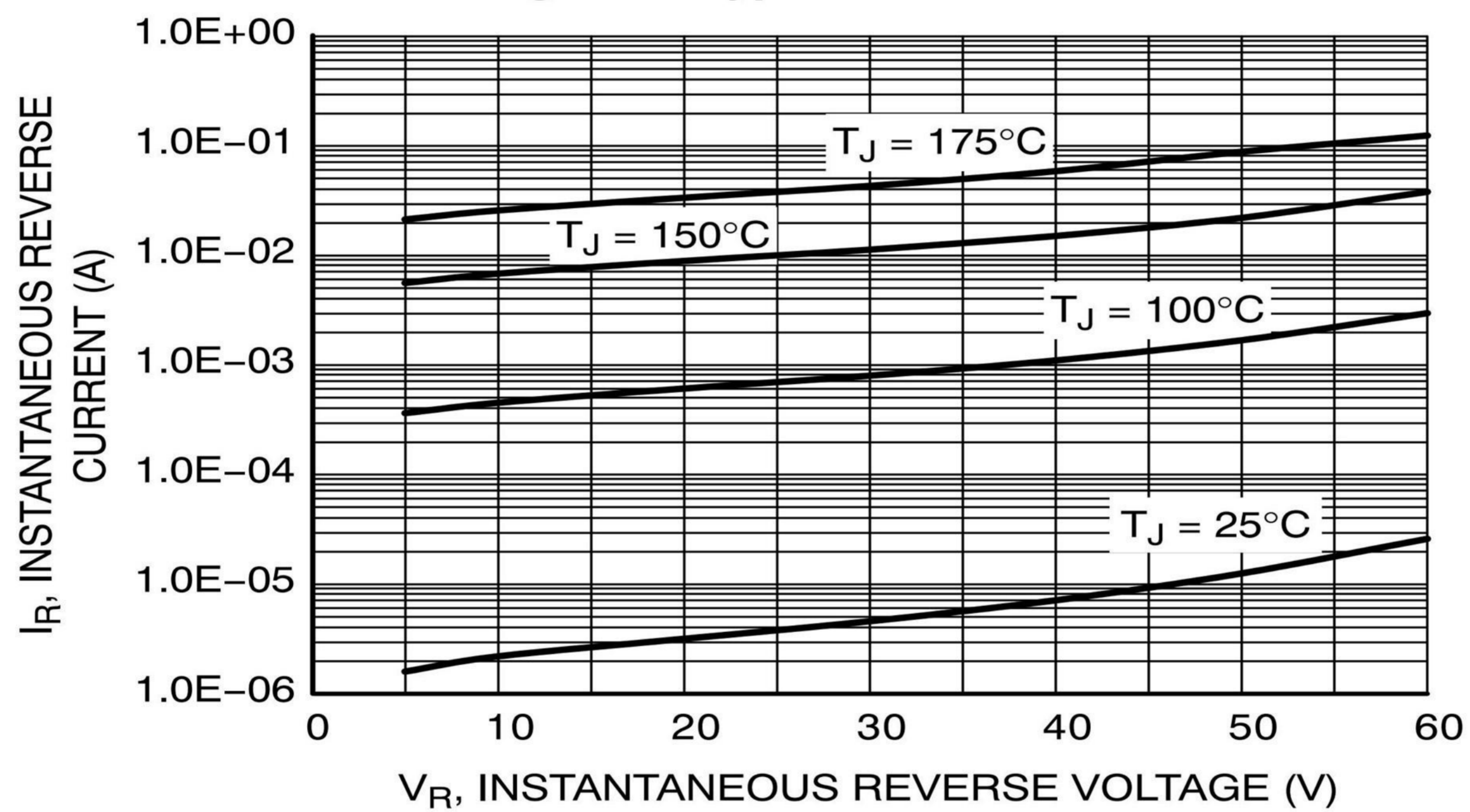
Figure 4. Maximum Reverse Current
