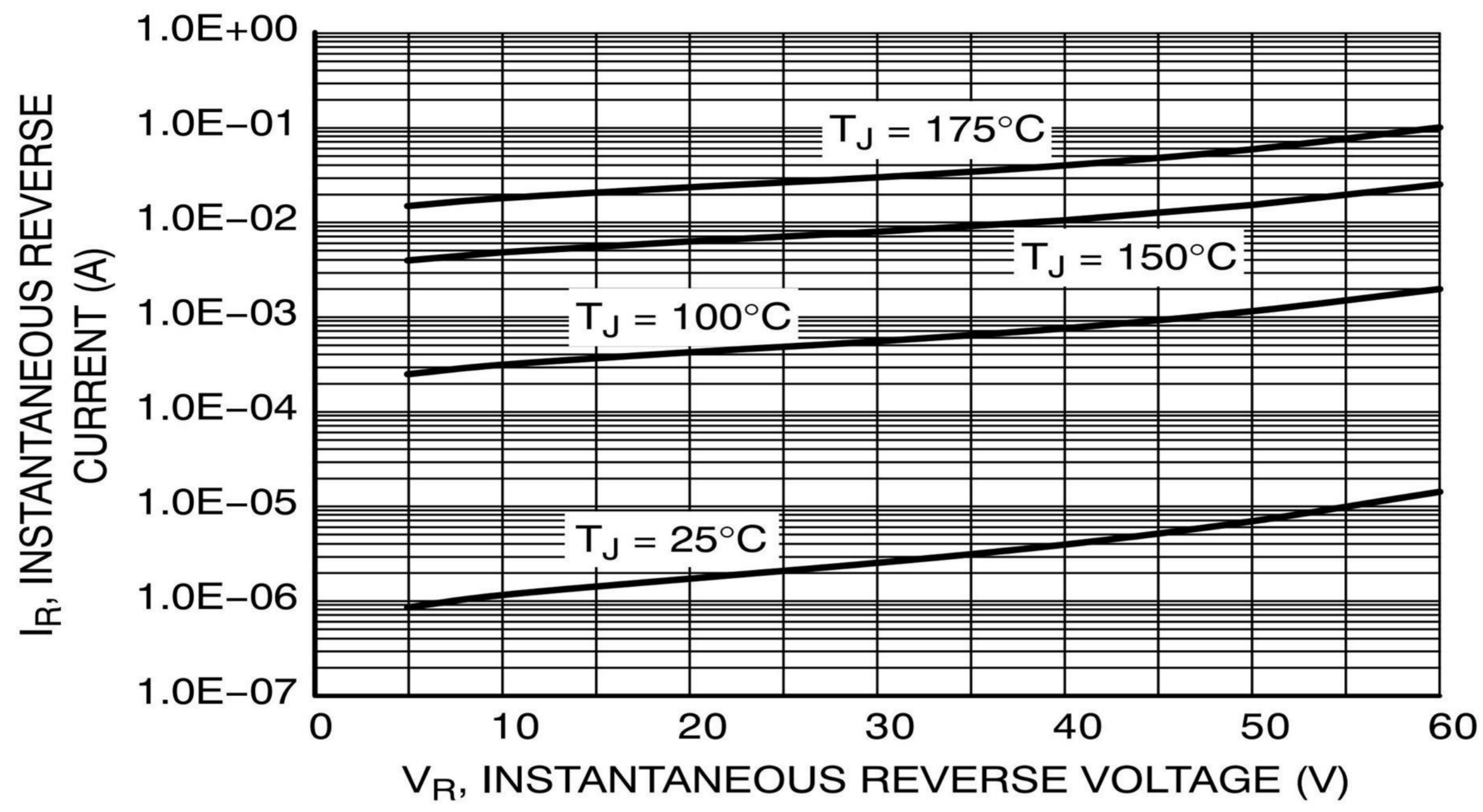
Figure 3. Typical Reverse Current
