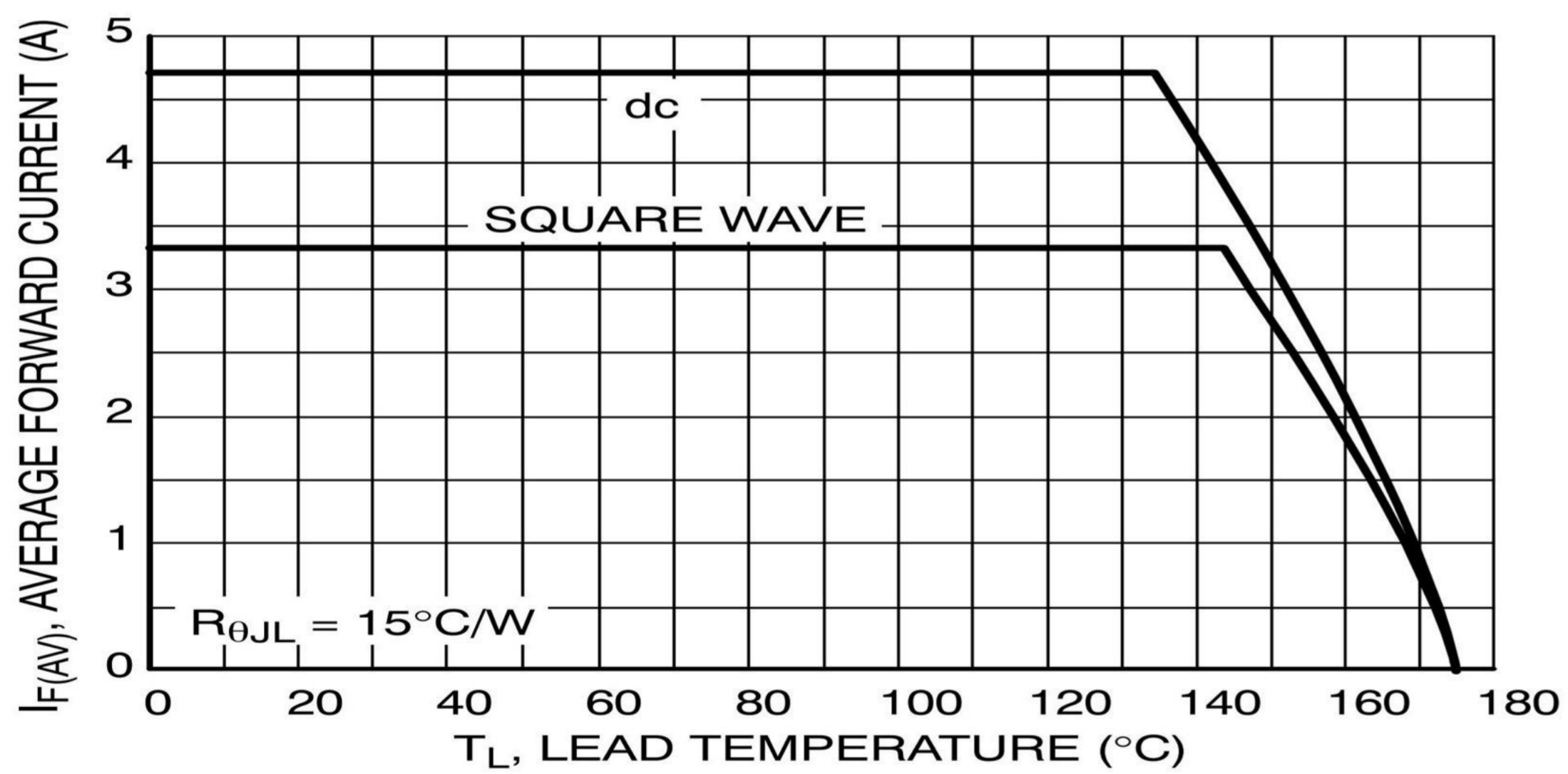
Figure 5. Current Derating
