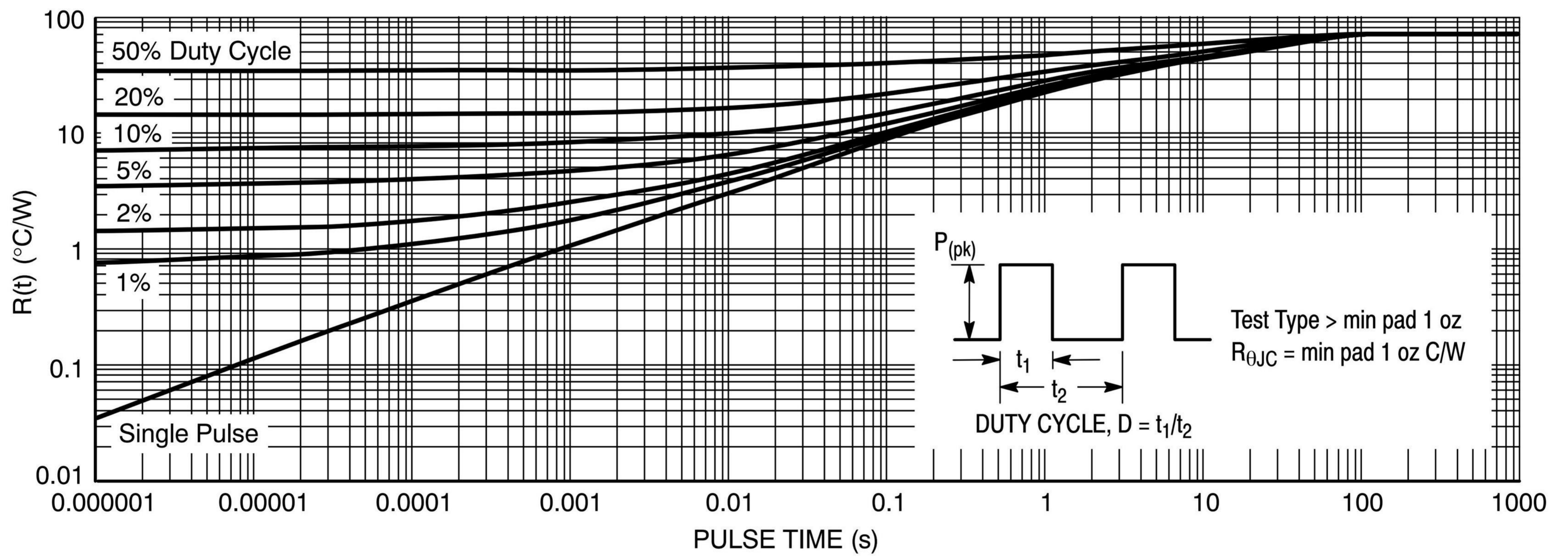
Figure 9. Typical Thermal Response, Junction-to-Ambient, SMB Package
