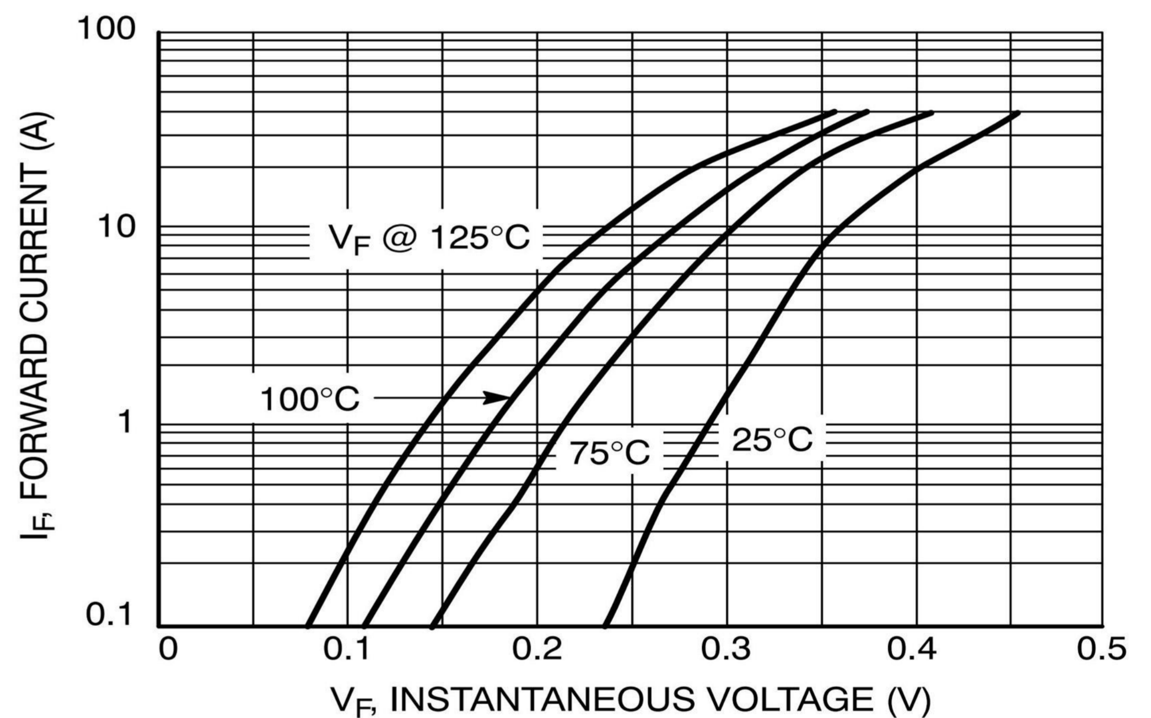
Figure 2. Maximum Forward Voltage
