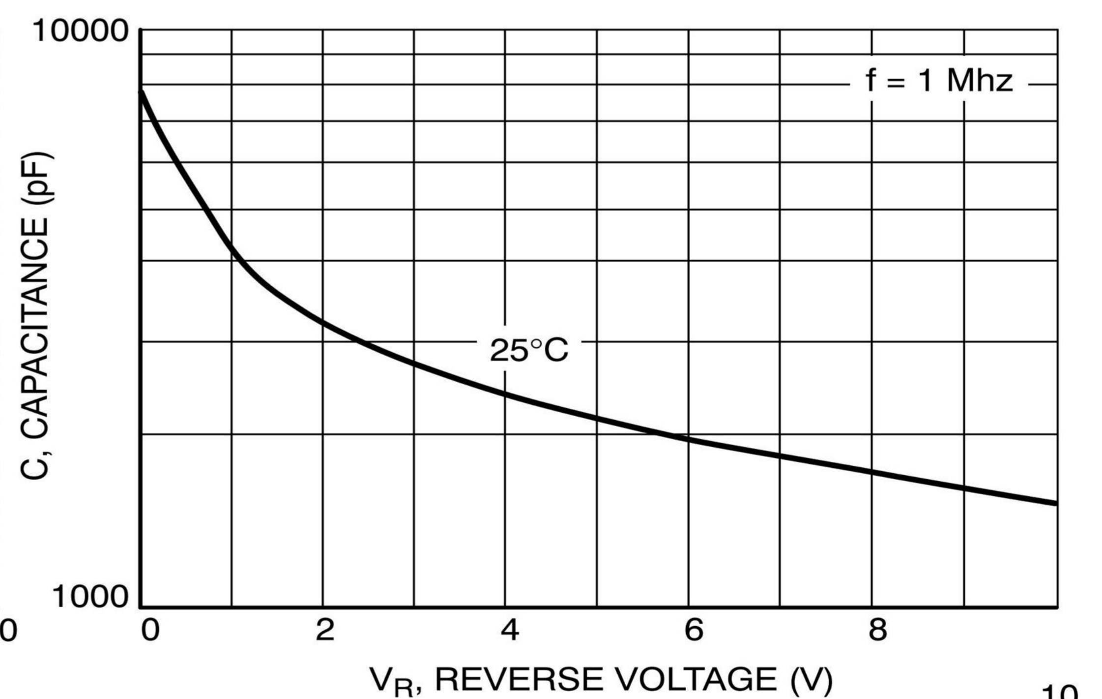
Figure 4. Typical Capacitance
