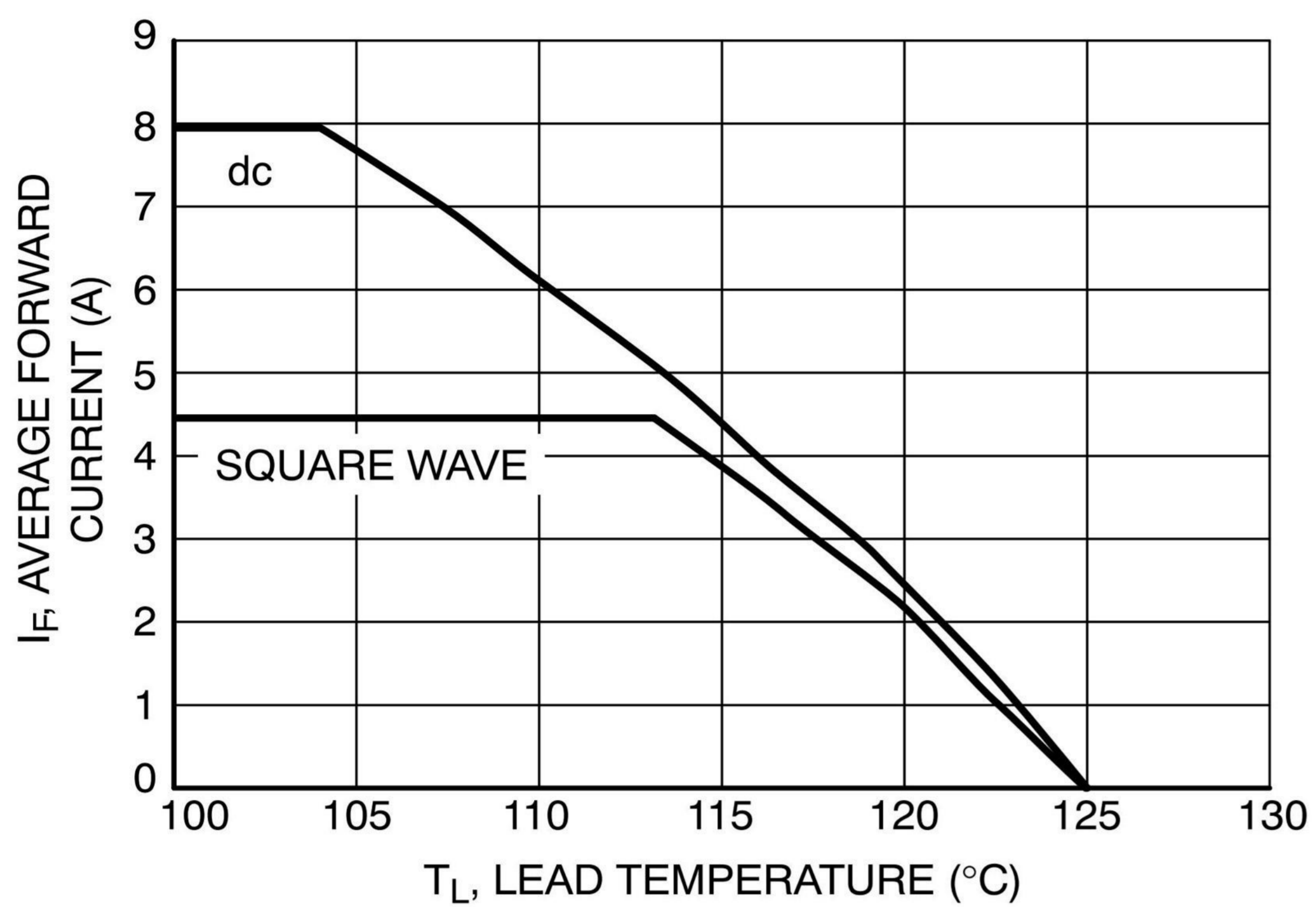
Figure 5. Current Derating (Junction-to-Lead)
