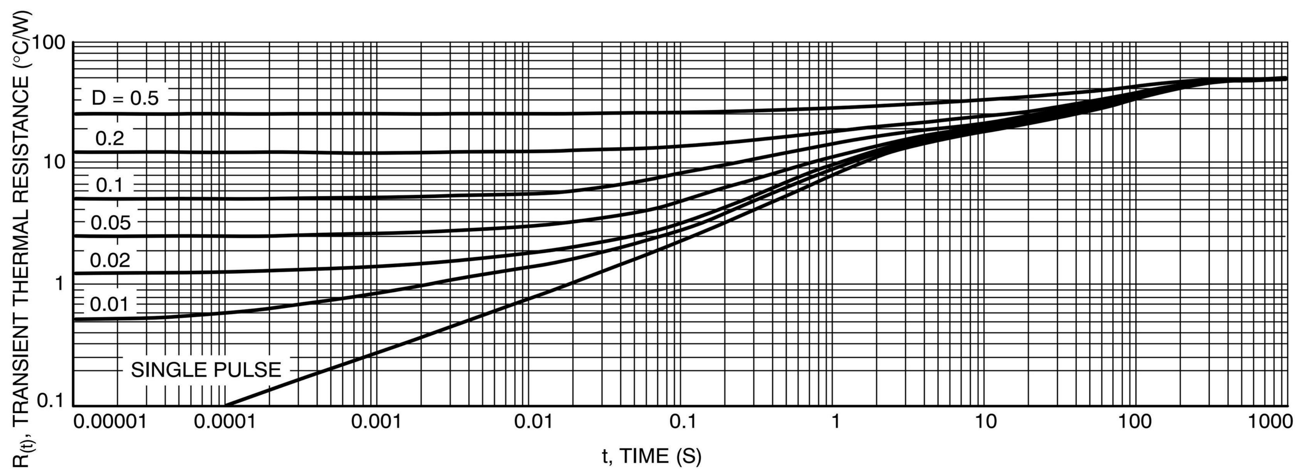
Figure 8. Thermal Response, Junction-to-Ambient (1 inch pad)
