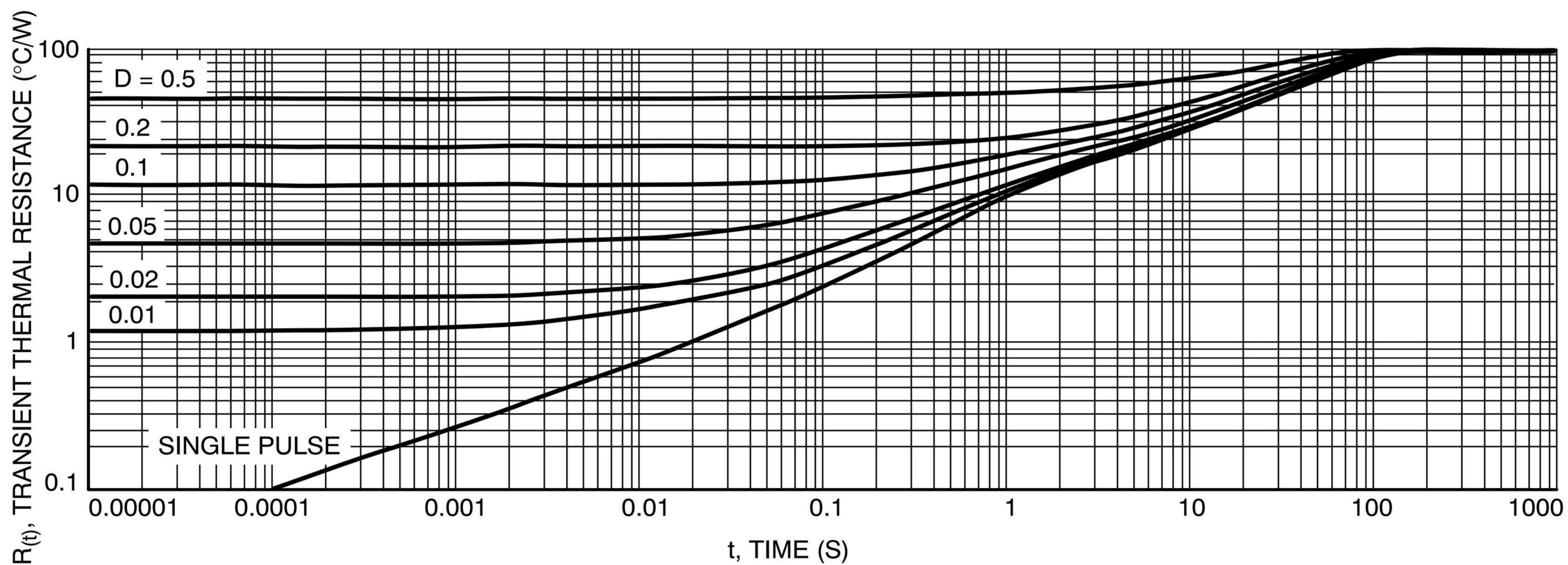
Figure 7. Thermal Response, Junction-to-Ambient (min pad)
