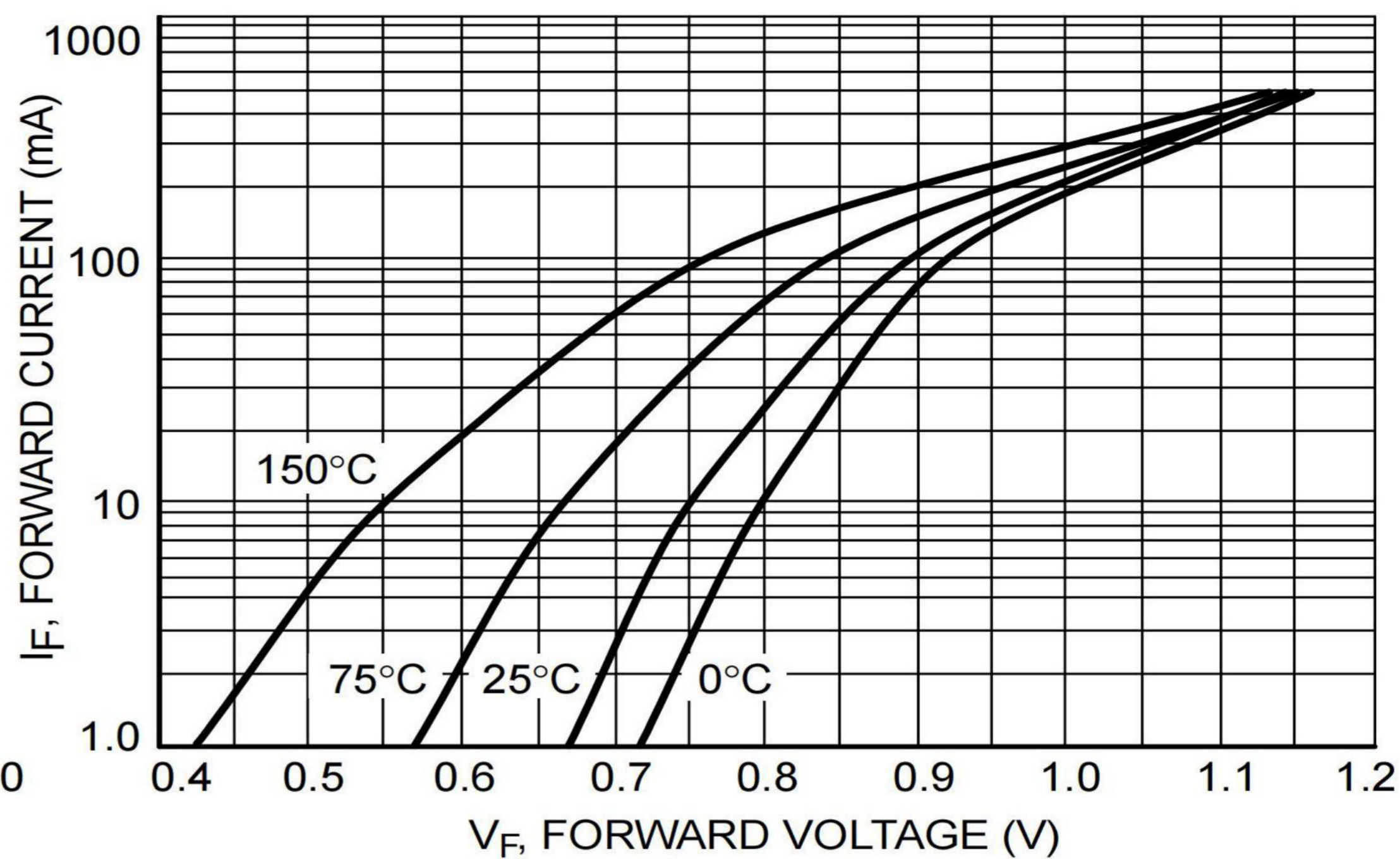
Figure 2. Typical Forward Voltage
