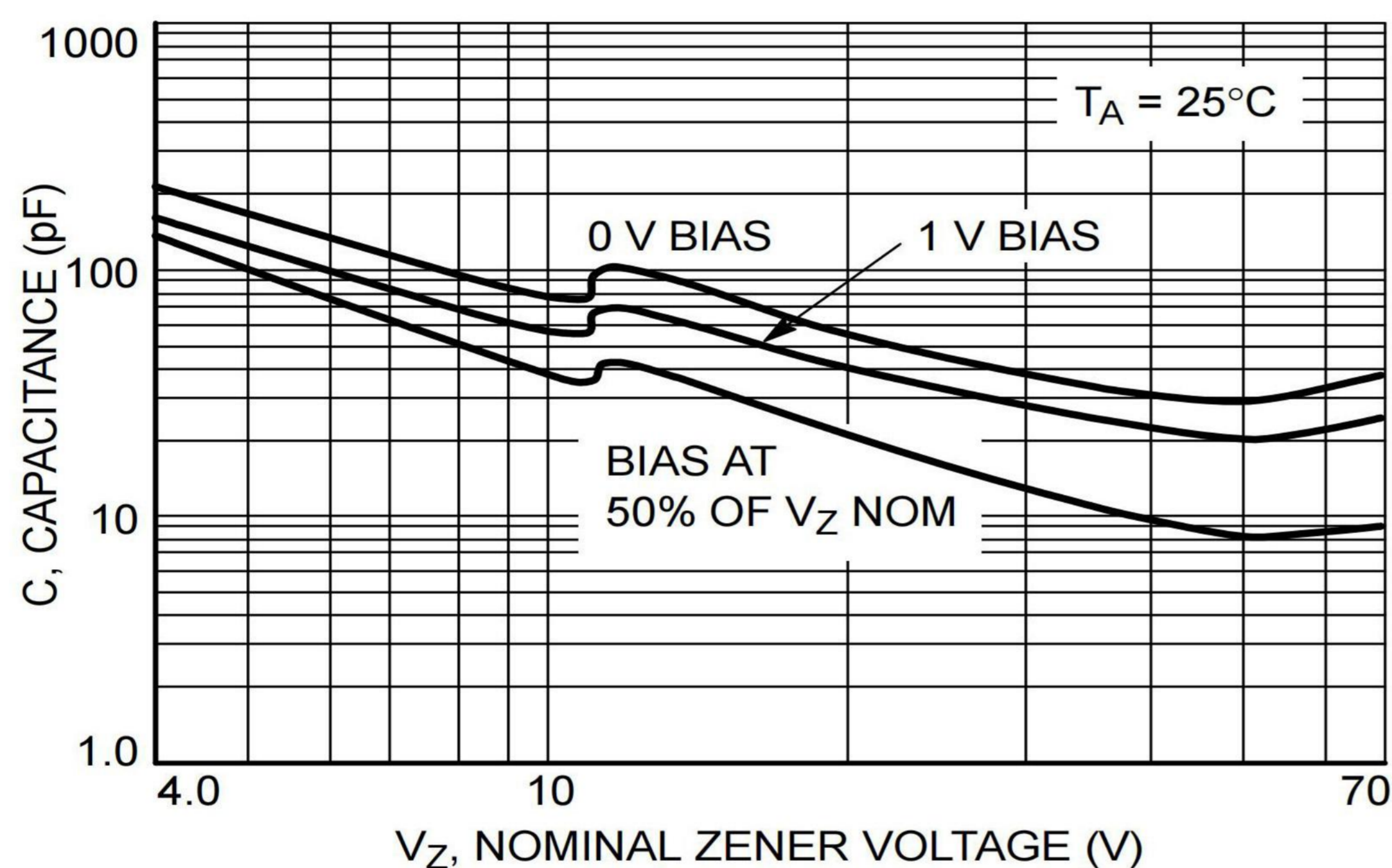
Figure 3. Typical Capacitance
