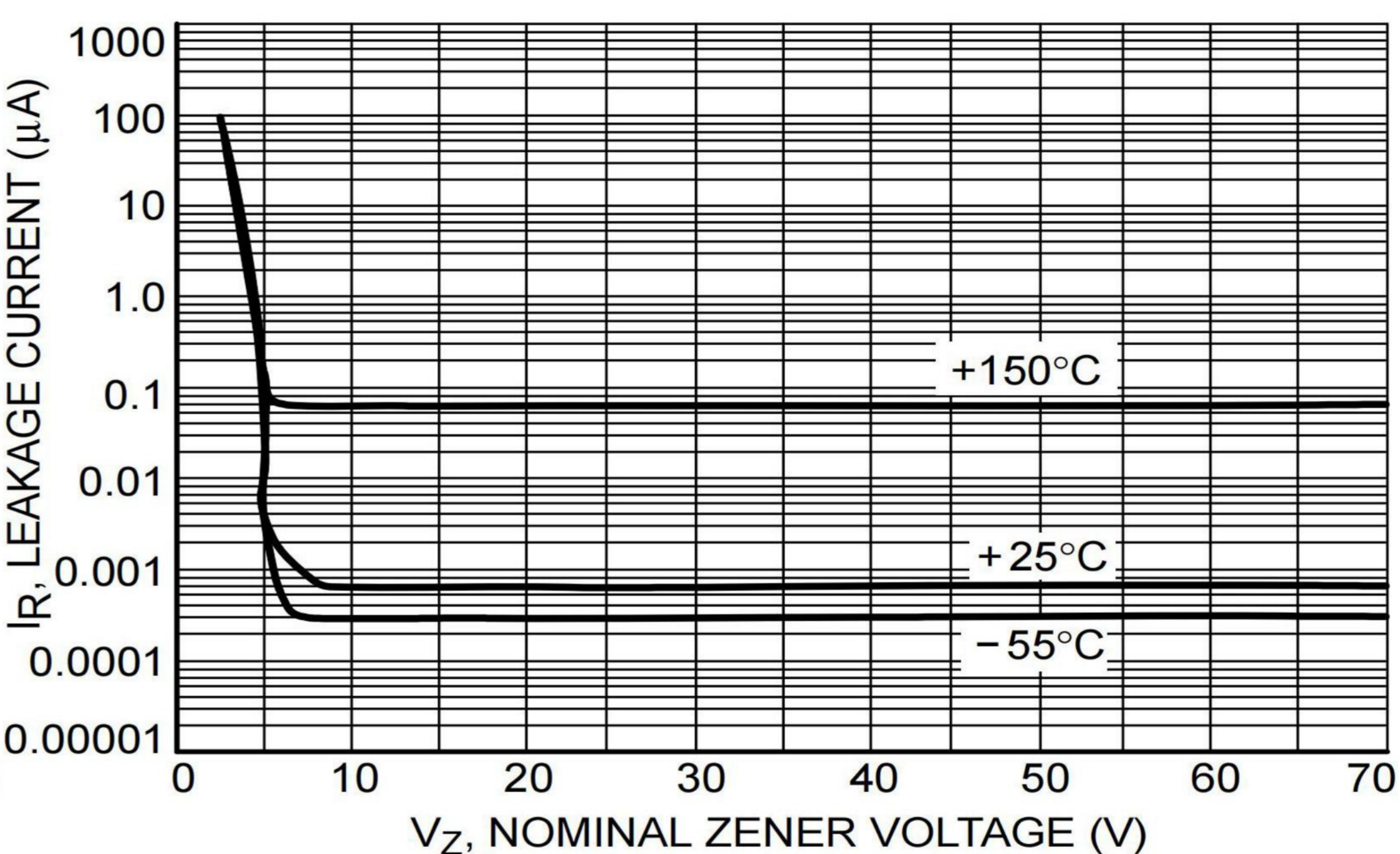
Figure 4. Typical Leakage Current
