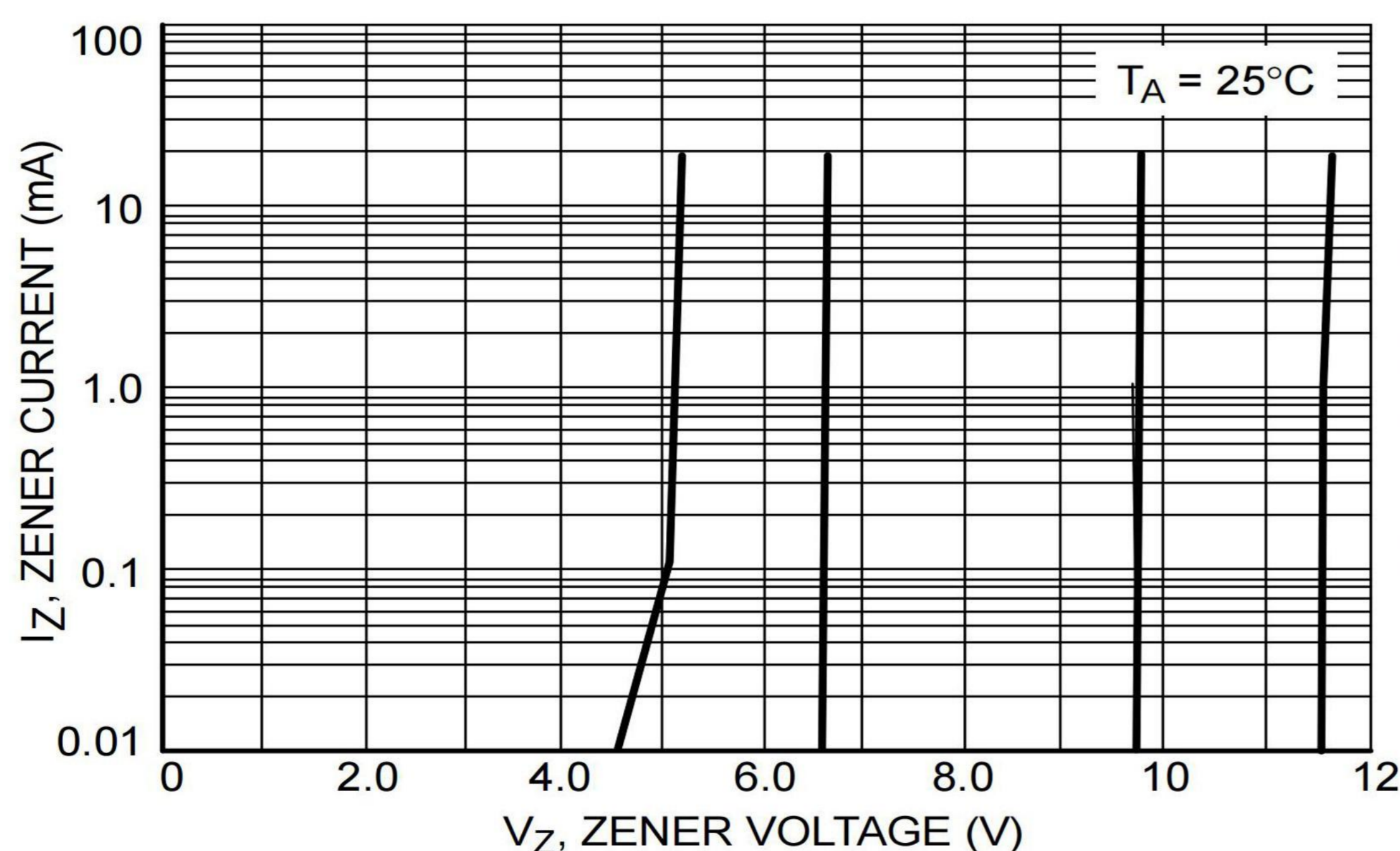
Figure 5. Zener Voltage versus Zener Current (V Z Up to 12 V)
