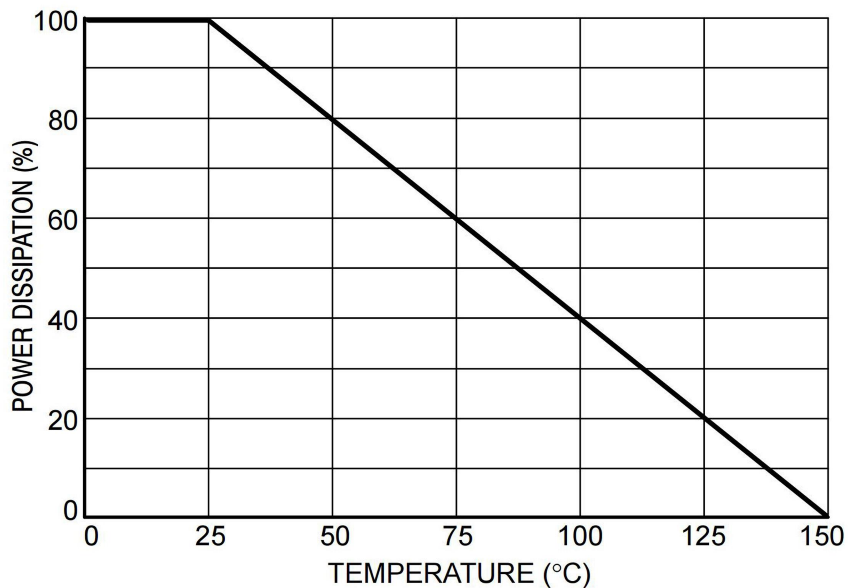
Figure 7. Steady State Power Derating
