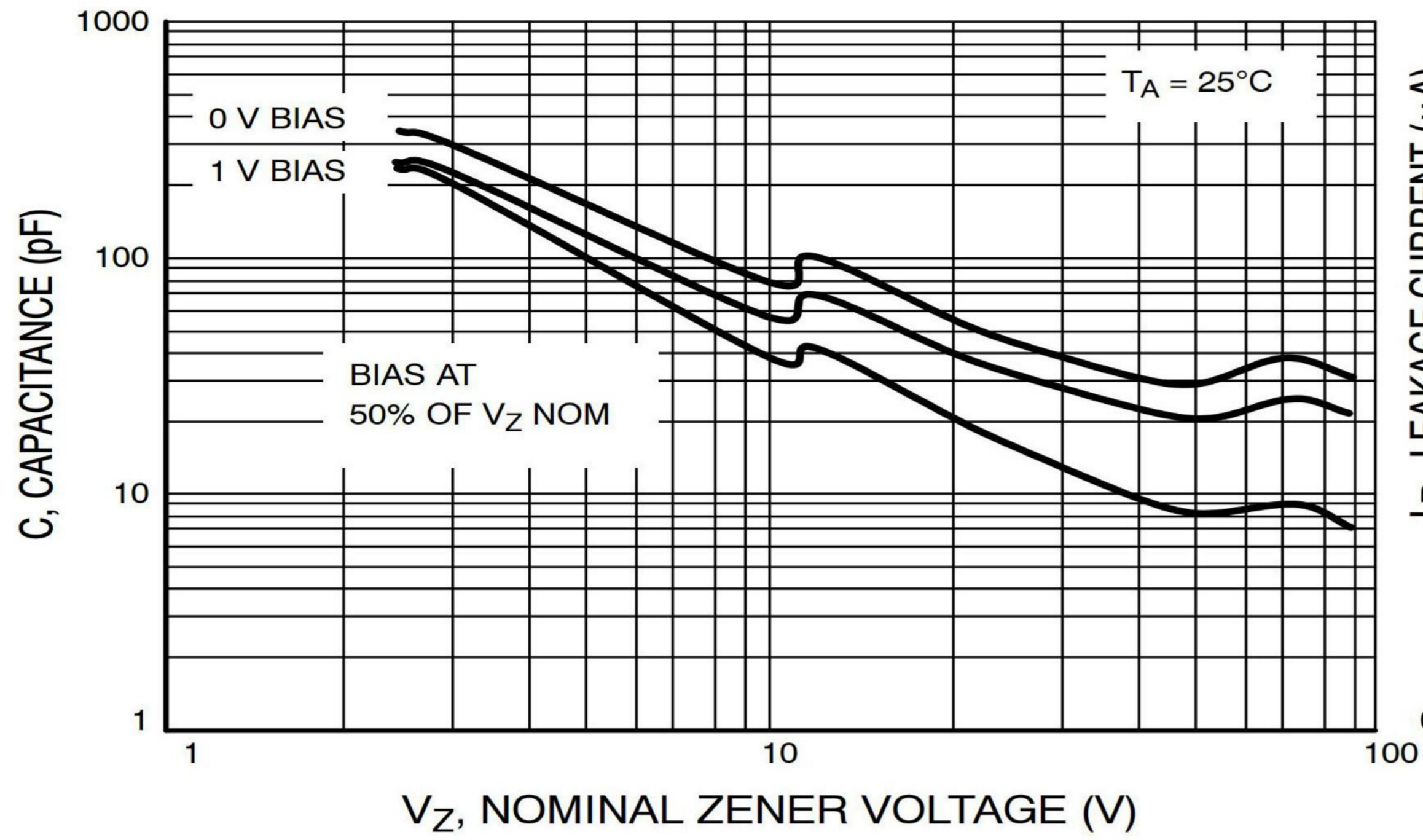
Figure 7. Typical Capacitance
