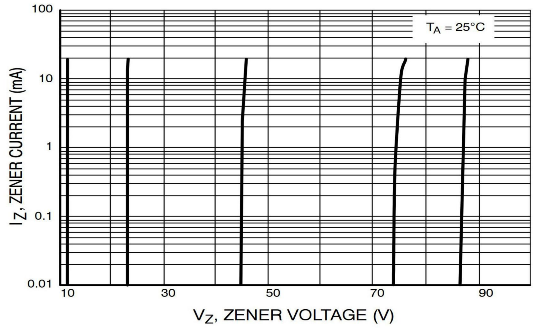
Figure 10. Zener Voltage versus Zener Current (12 V to 91 V)
