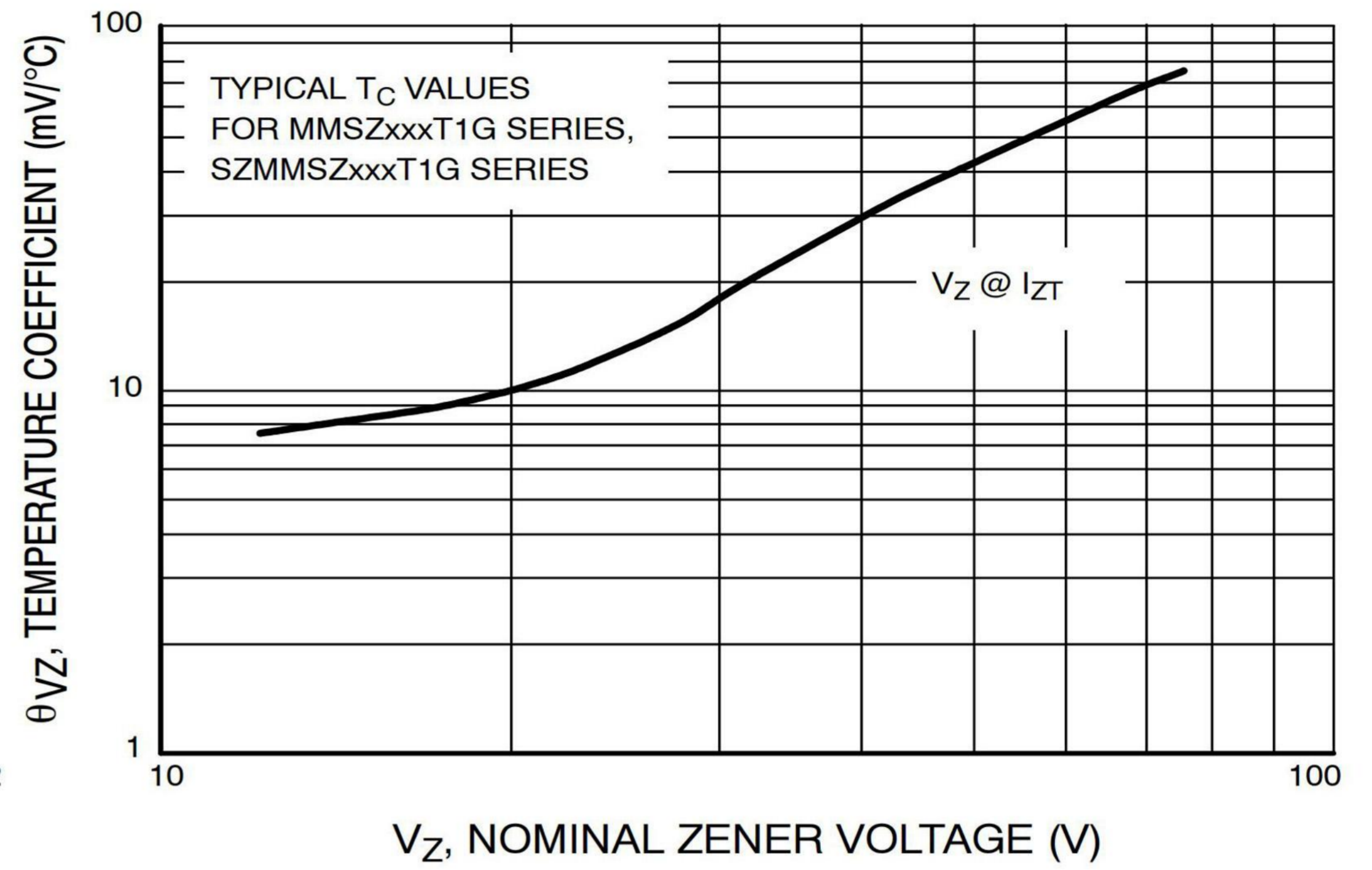
Figure 2. Temperature Coefficients (Temperature Range -55°C to +150°C)
