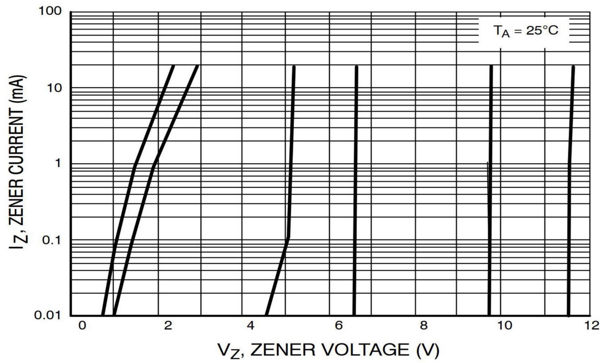
Figure 9. Zener Voltage versus Zener Current ( V_Z Up to 12 V)
