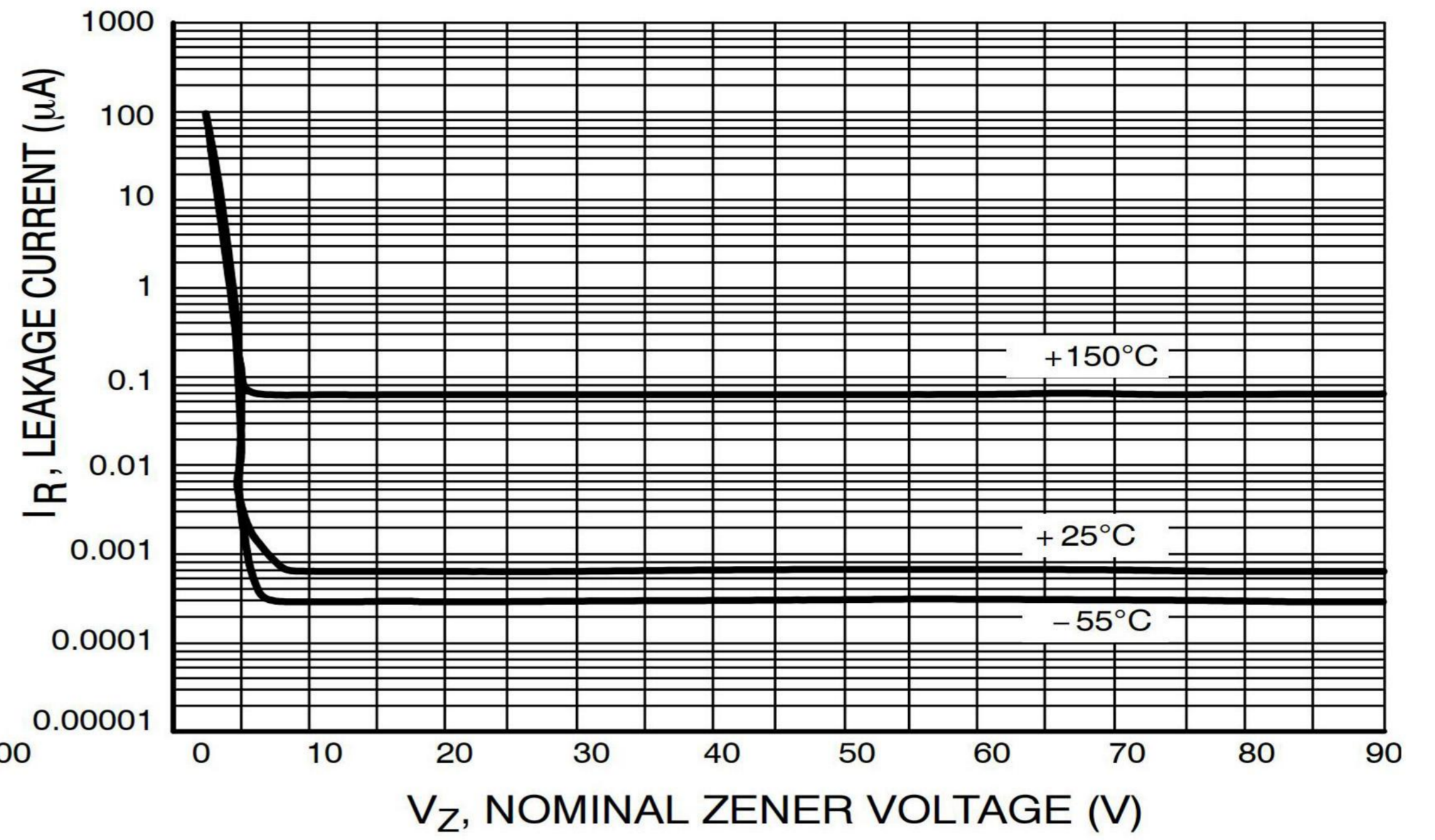
Figure 8. Typical Leakage Current
