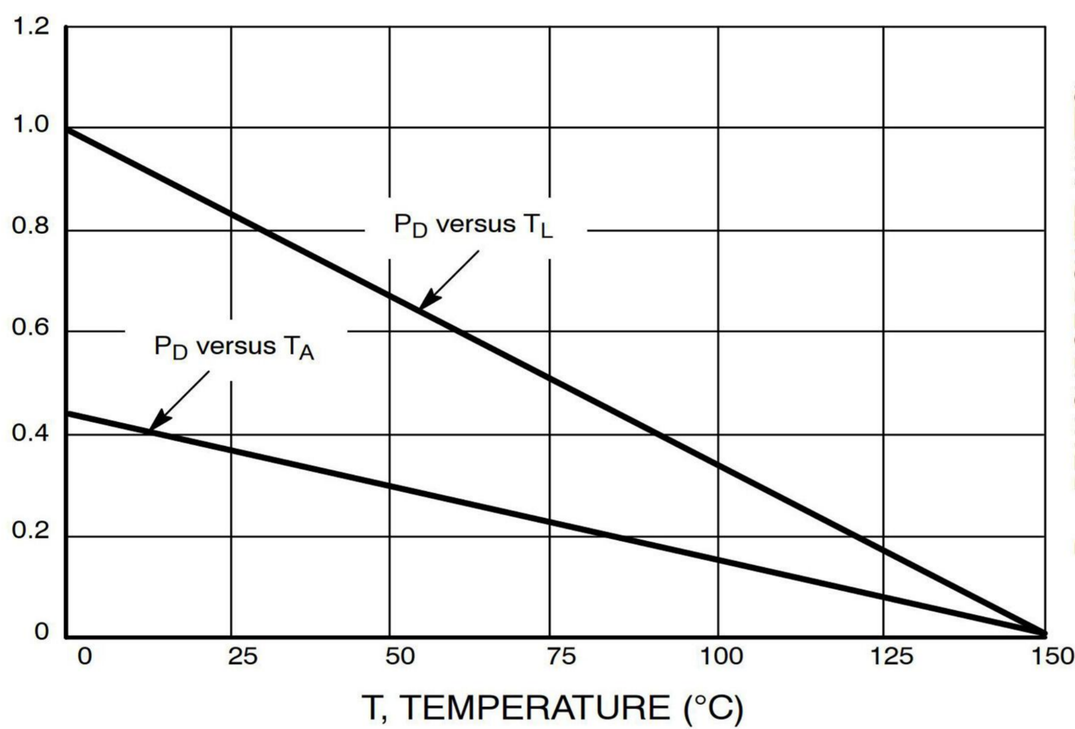
Figure 3. Steady State Power Derating
