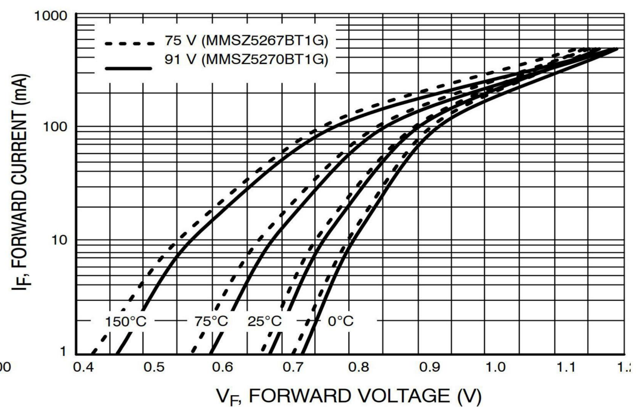
Figure 6. Typical Forward Voltage
