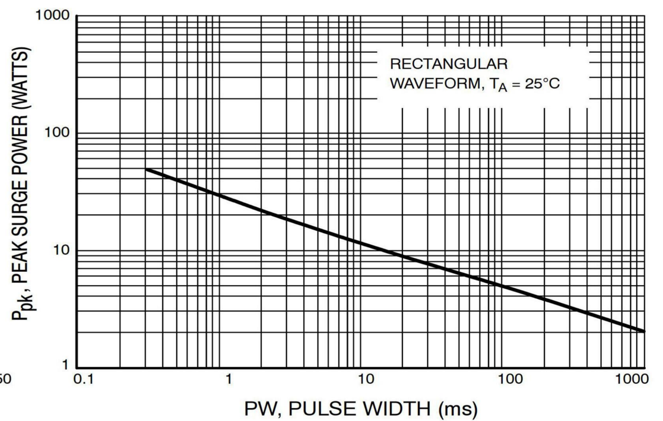
Figure 4. Maximum Nonrepetitive Surge Power
