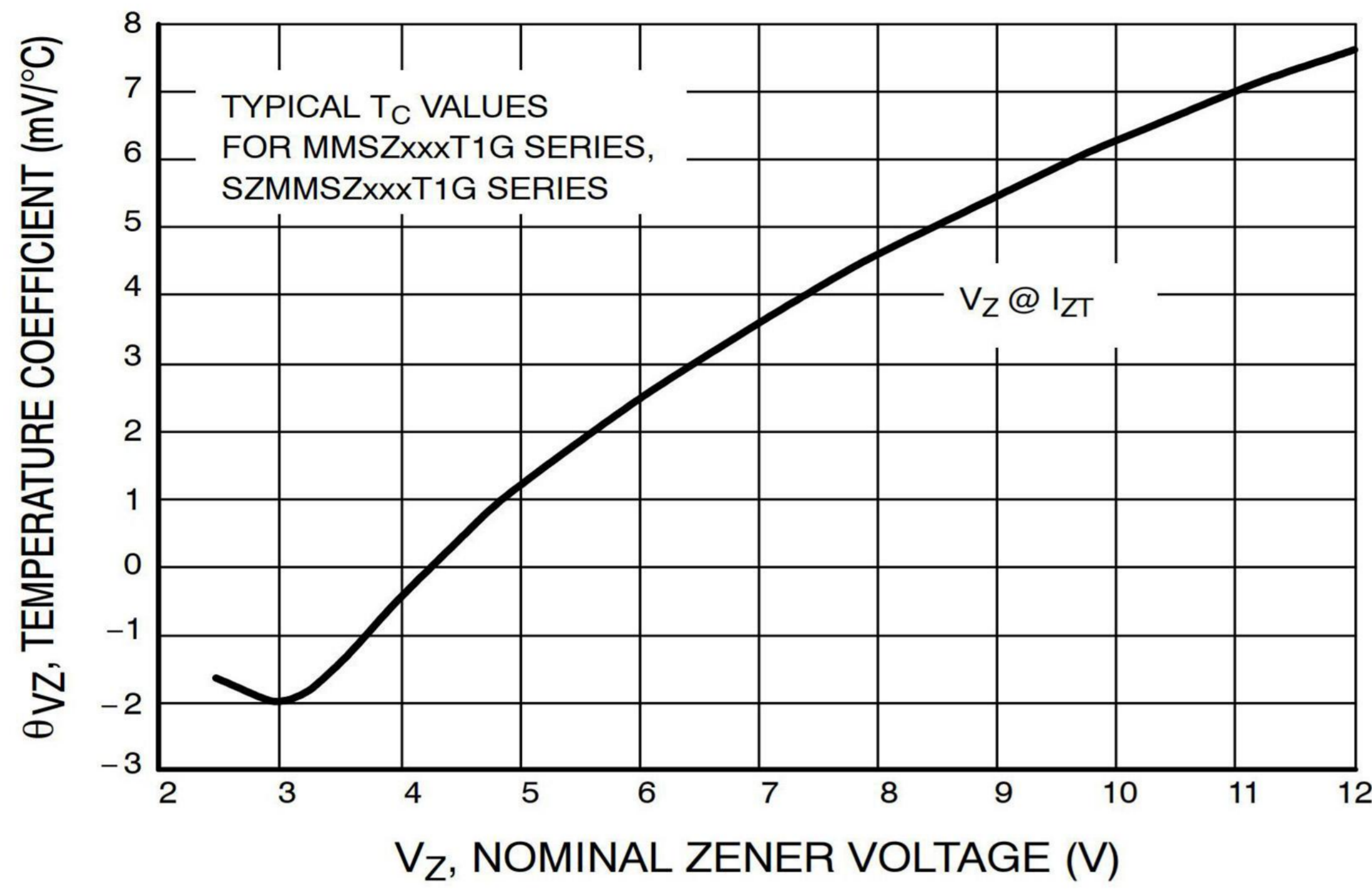
Figure 1. Temperature Coefficients (Temperature Range -55°C to +150°C)
