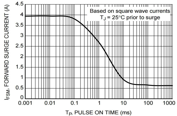
Figure 4. Forward Surge Current
