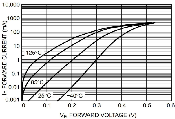
Figure 1. Forward Voltage
