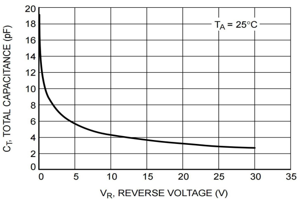
Figure 3. Total Capacitance
