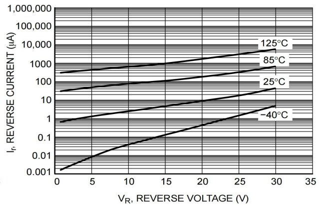
Figure 2. Leakage Current
